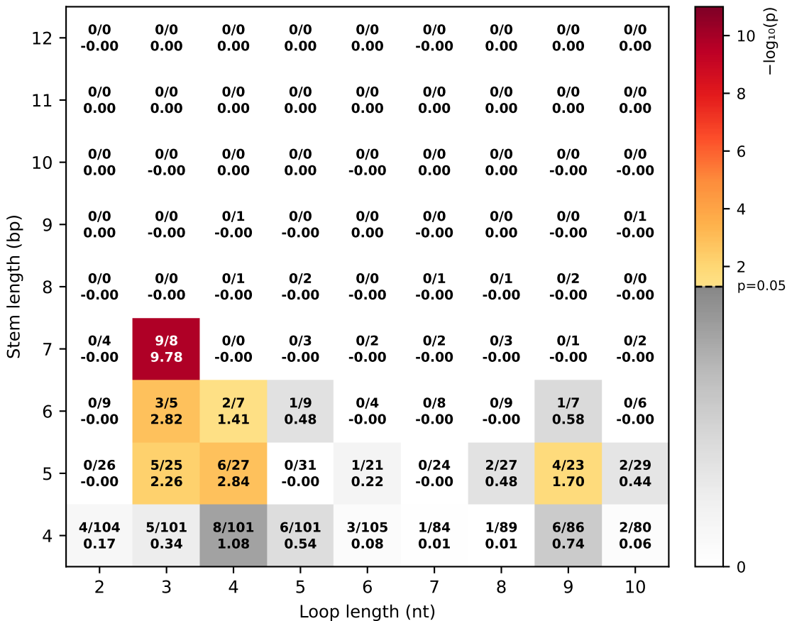
TC at the 3' loop end / All hairpins
