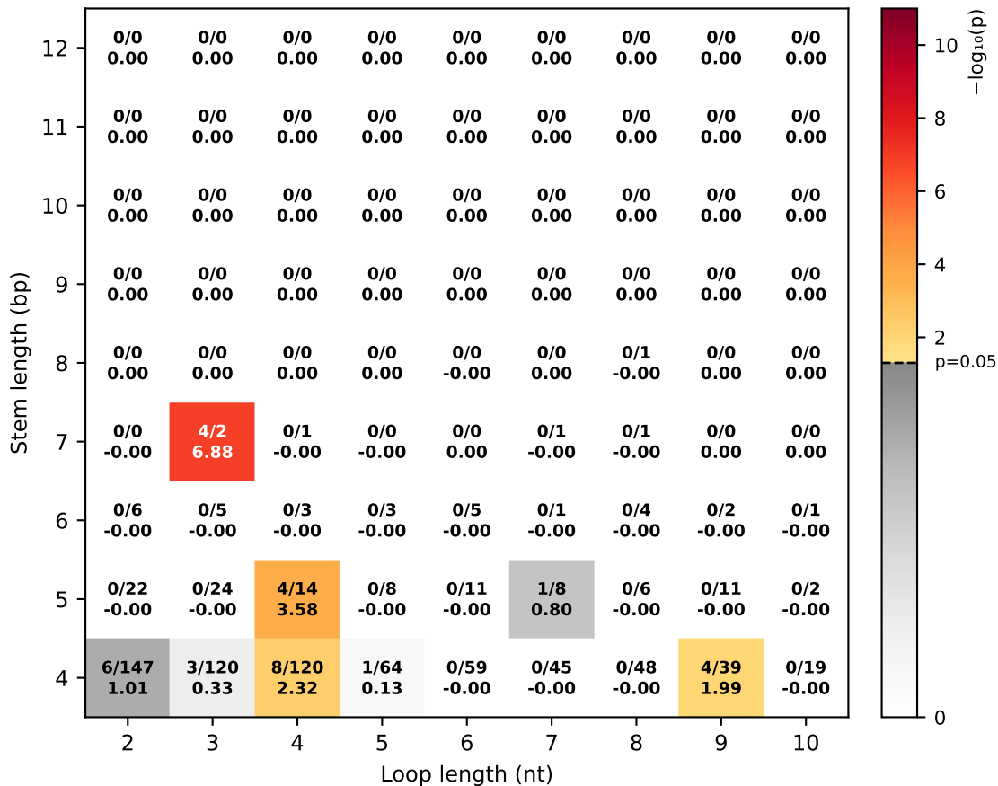
C at the 3' loop end / Minimum coverage
