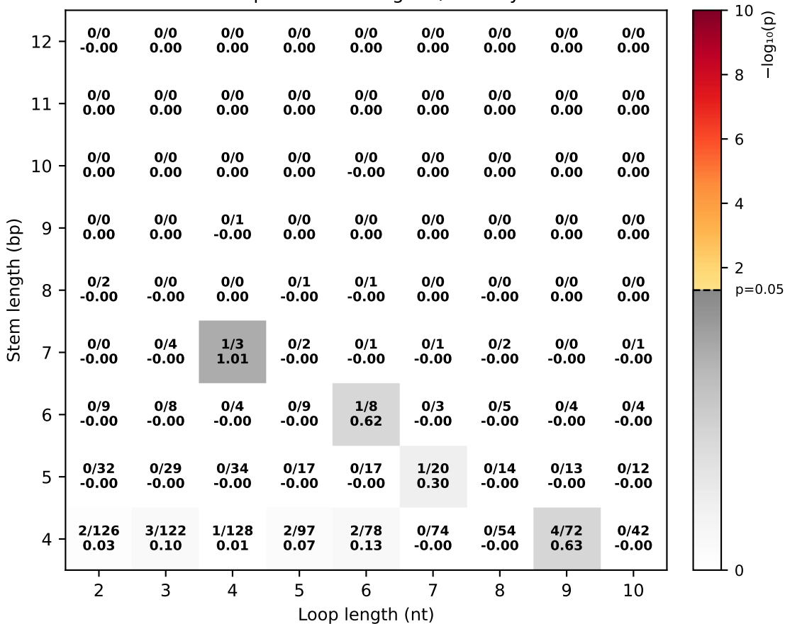
C at the 3' loop end excluding TC / Greedy selection
