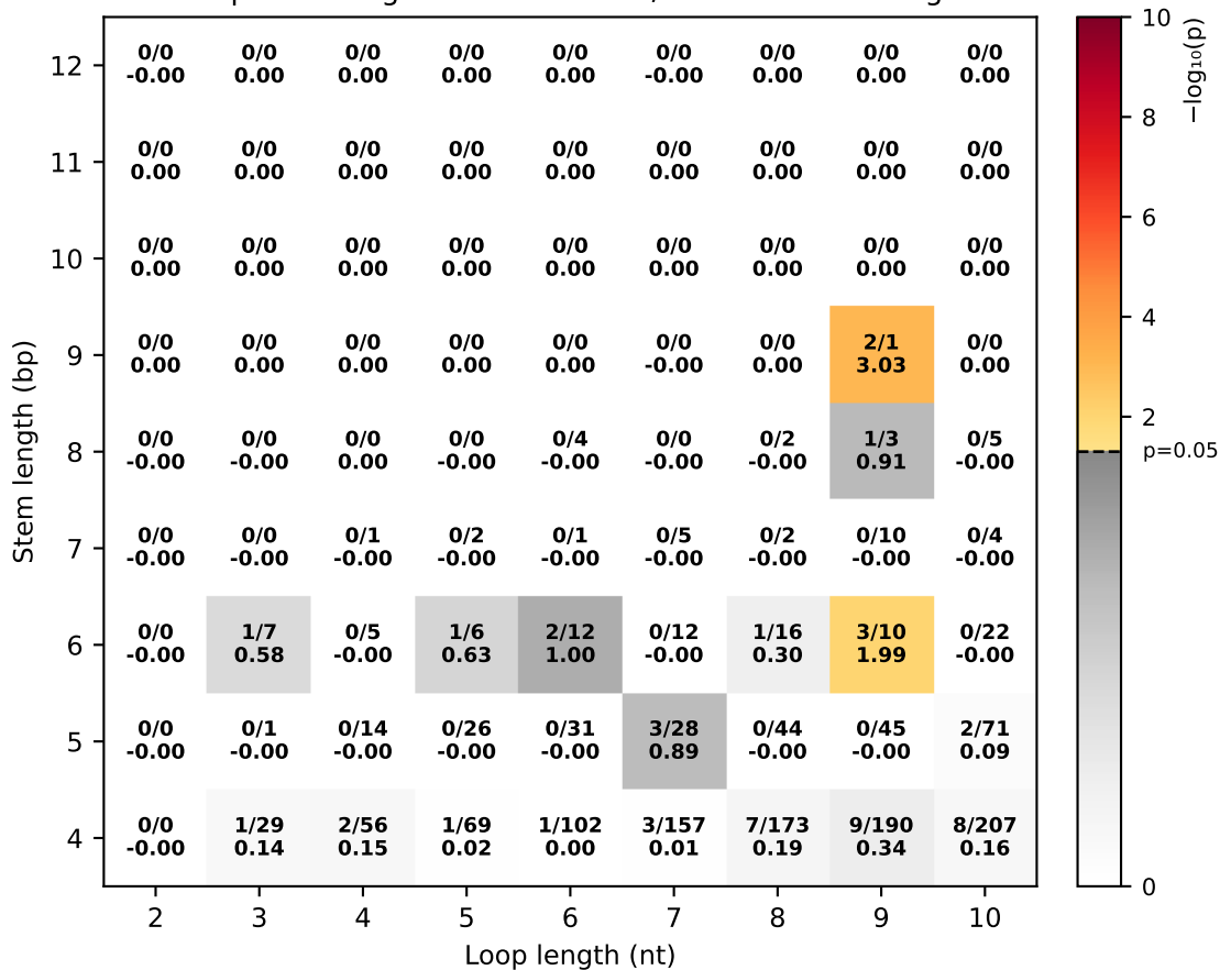
Loop excluding TC at the 3' end / Maximum coverage
