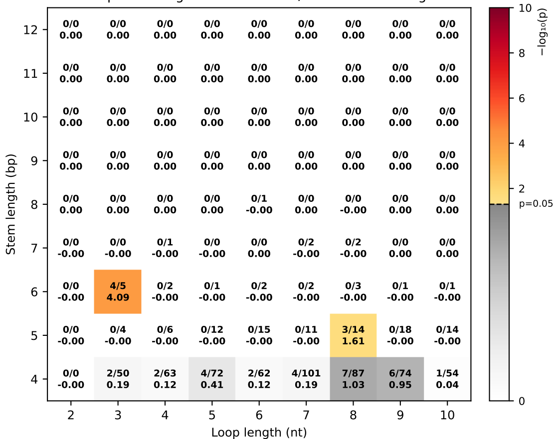
Loop excluding TC at the 3' end / Minimum coverage
