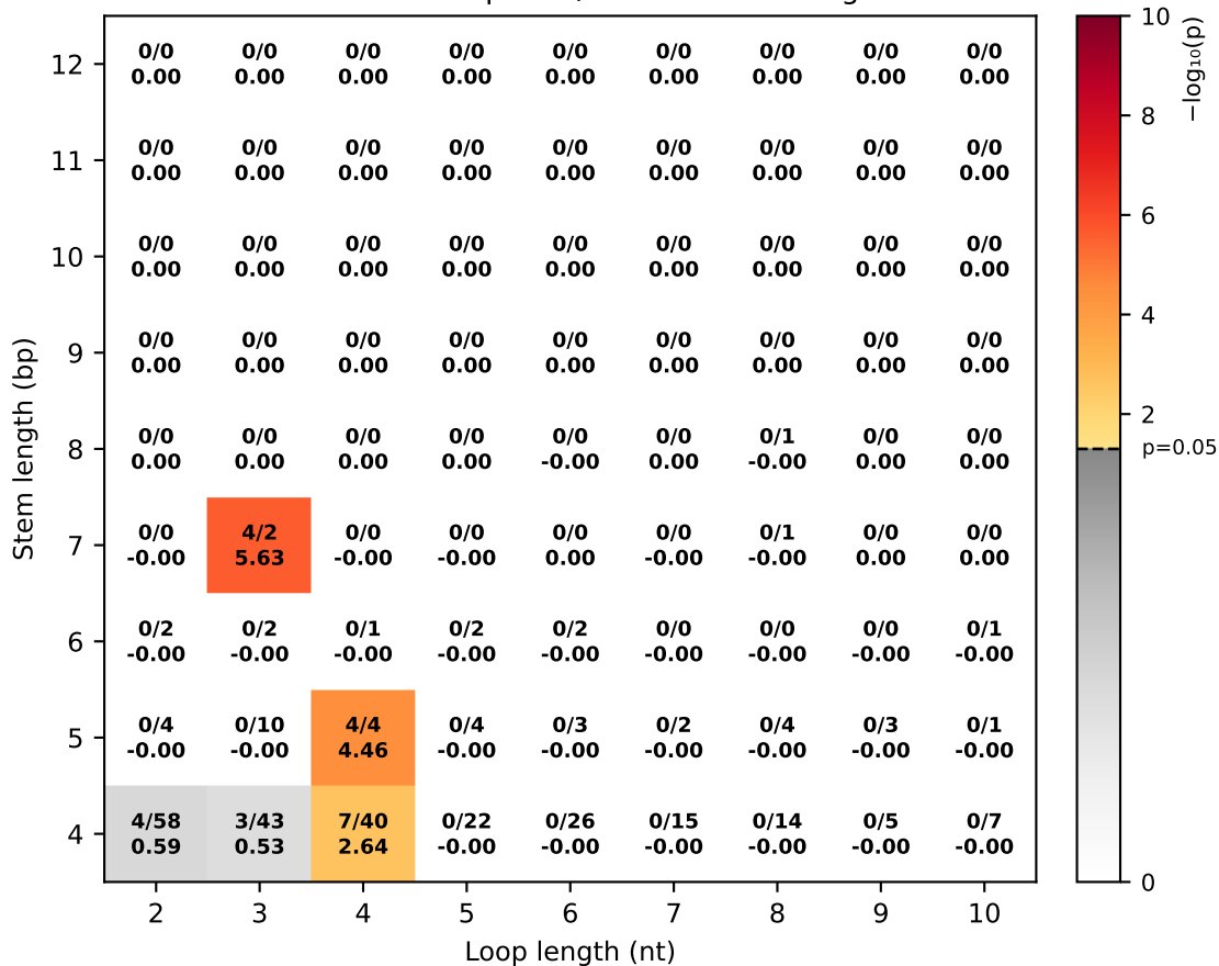
TC at the 3' loop end / Minimum coverage
