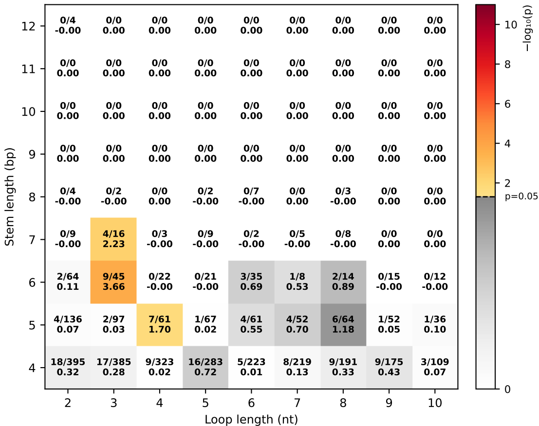
Whole hairpin / Most stable hairpin
