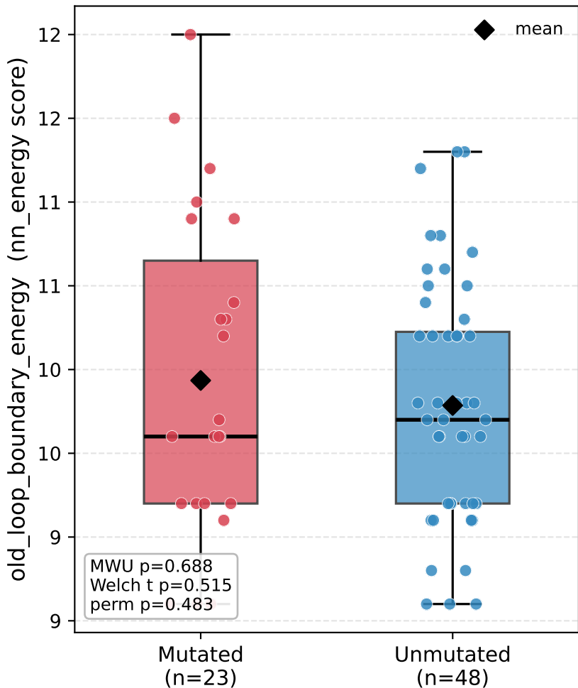
All (stem, loop) shapes pooled -- old (nn_energy) score
