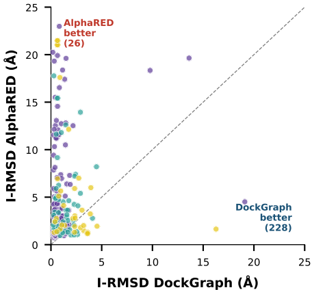
I-RMSD Comparison
