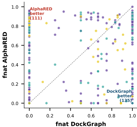
fnat Comparison
