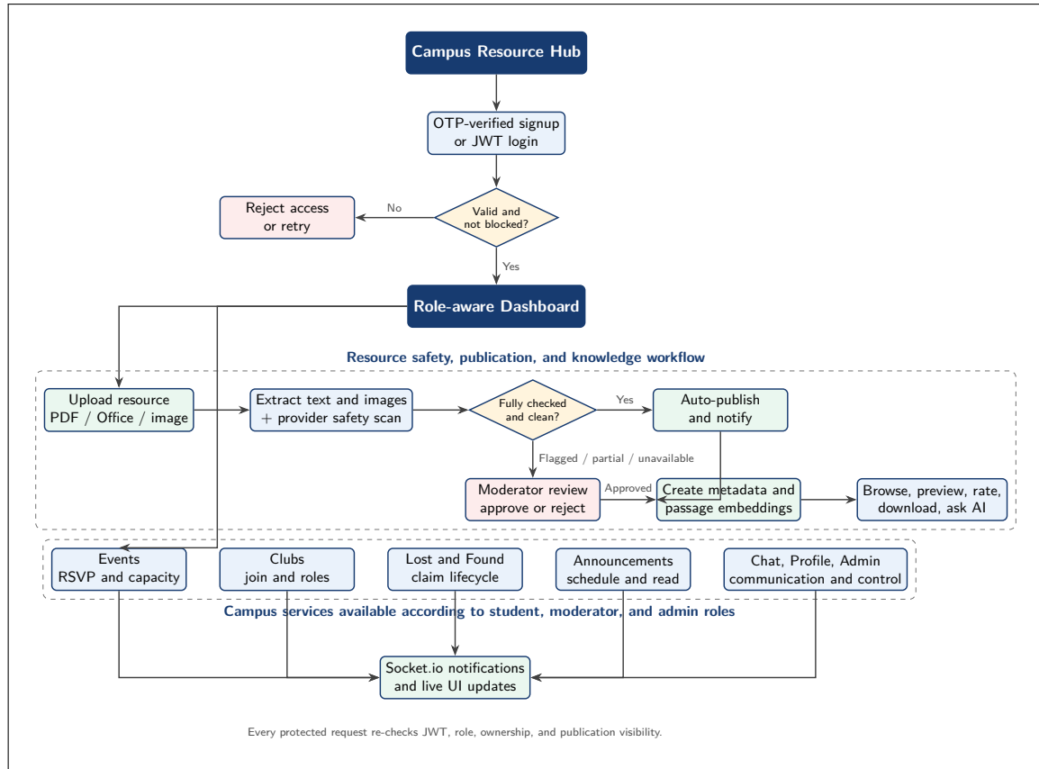
Figure 3.2: Overall system workflow, simplified from the project’s detailed draw.io design
