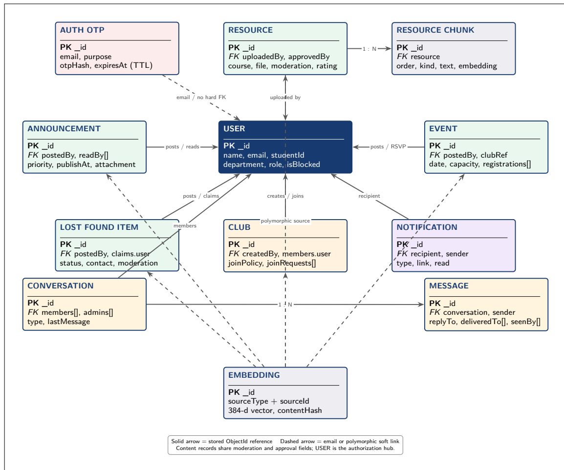
Figure 3.3: Entity-relationship diagram of the twelve MongoDB collections, simplified from the draw.io design
