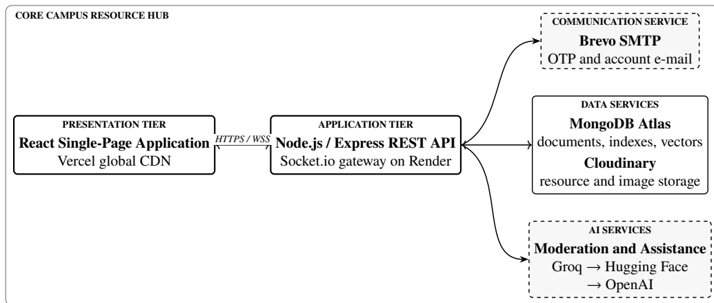
Figure 3.1: Three-tier system architecture, data services, and external integrations
