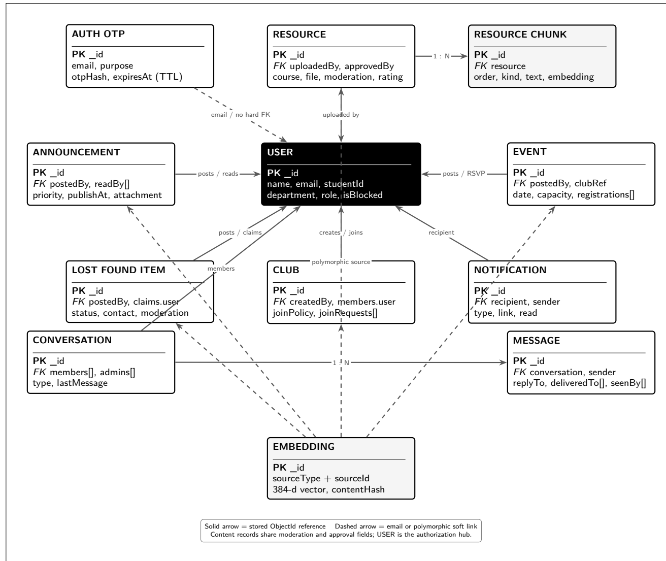
Figure 3.3: MongoDB collections for authorization, academic content, communication, and AI-assisted retrieval
