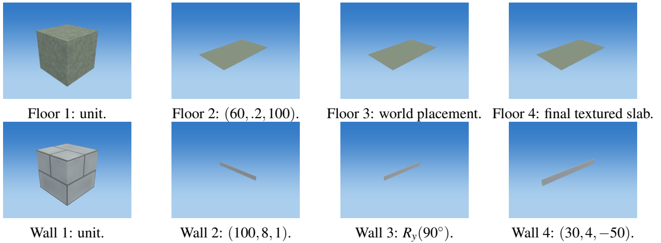
Figure 3: Arena parts are constructed from the shared cube. Scaling sets dimensions, rotation sets orientation, and translation places each component in the arena.
