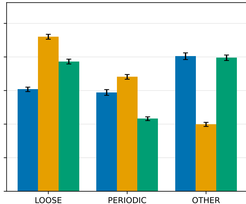
Sentence structure
