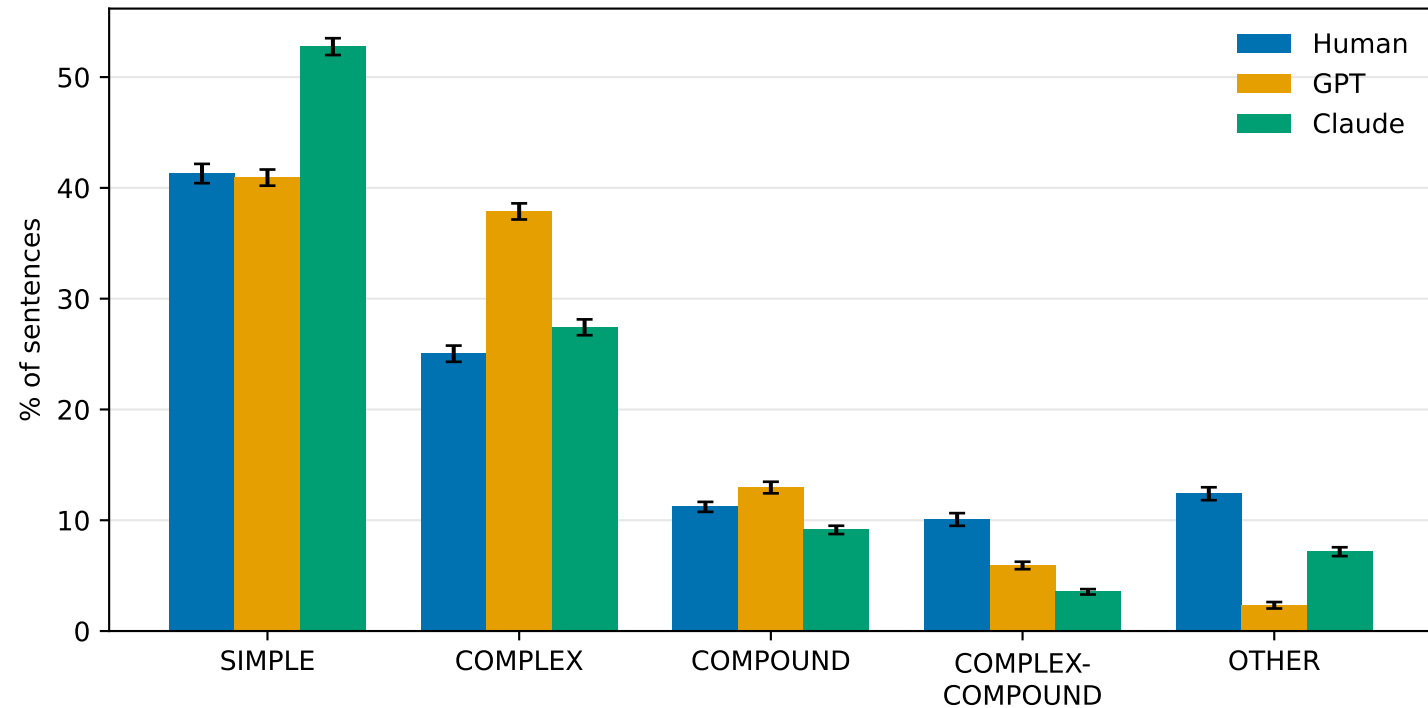
Sentence type
