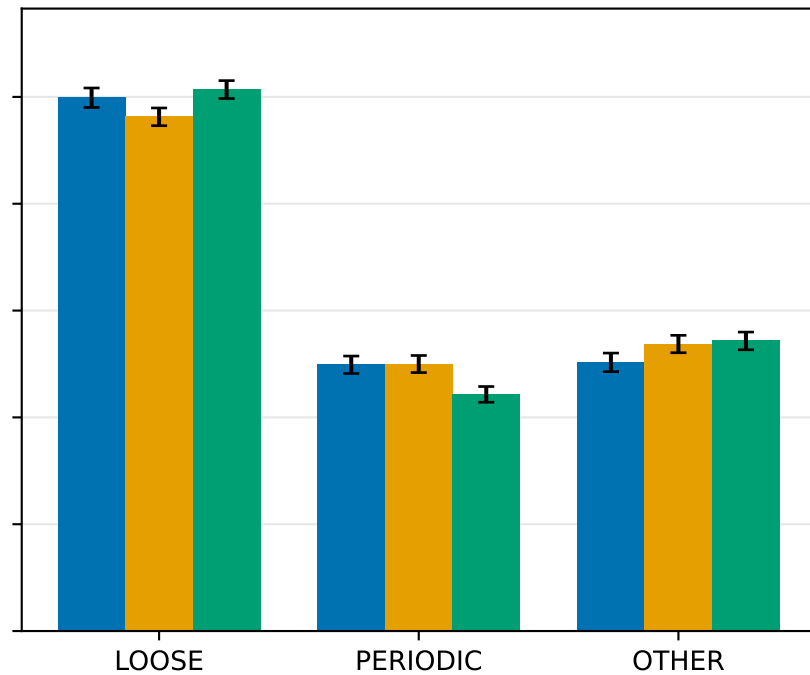
Sentence structure
