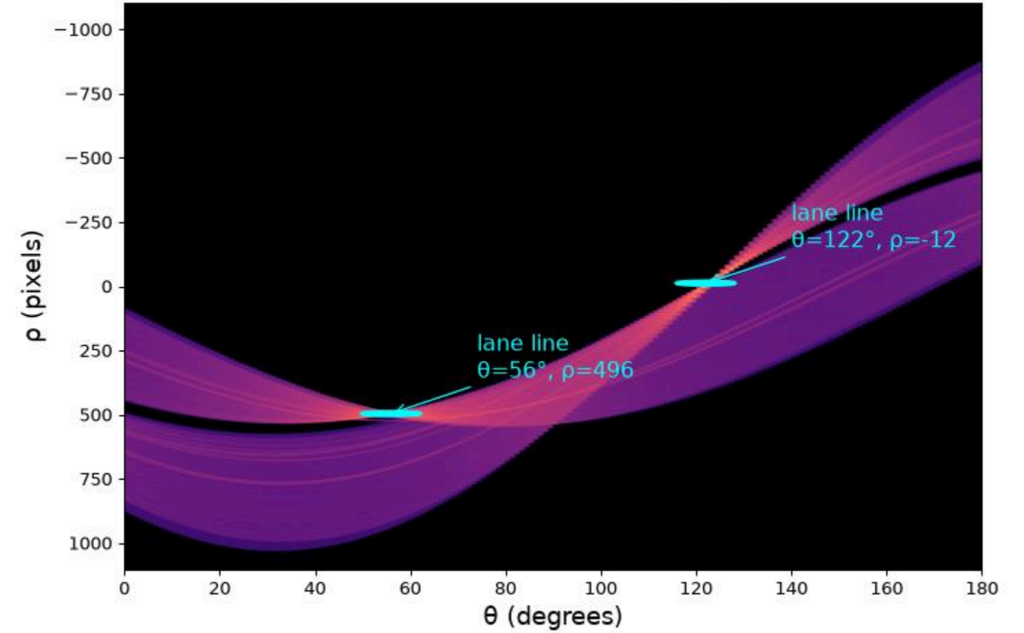
Hough accumulator: every edge pixel votes
