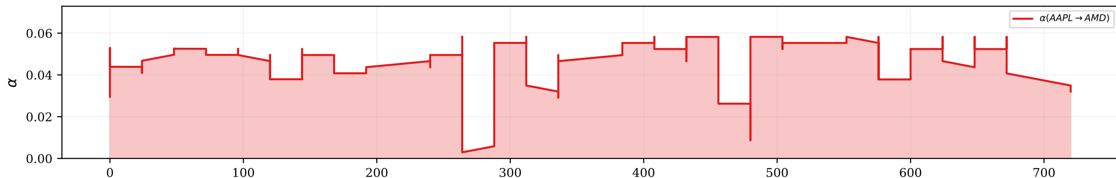
AAPL \rightarrow AMD (Semiconductors)
