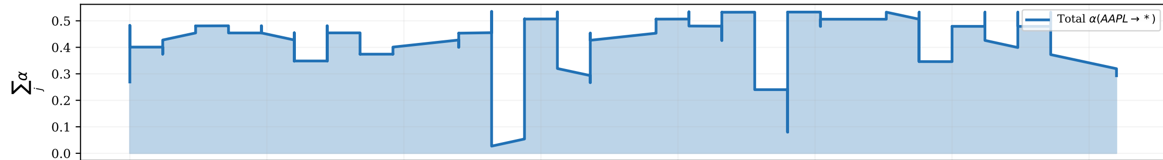
AAPL (Technology) — Total Outgoing Excitation
