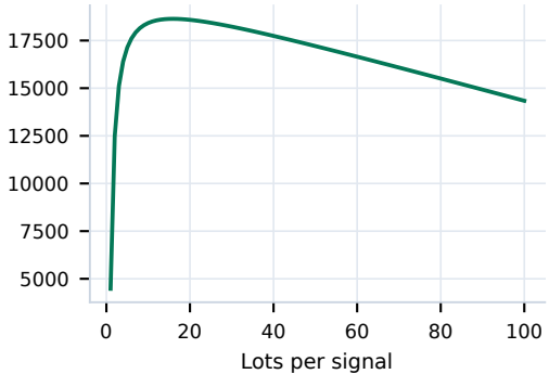
Equal-size capacity diagnostic
