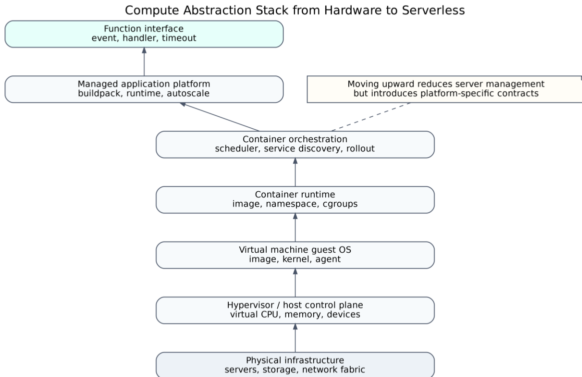
Figure 2.1: Compute Abstraction Stack from Hardware to Serverless
