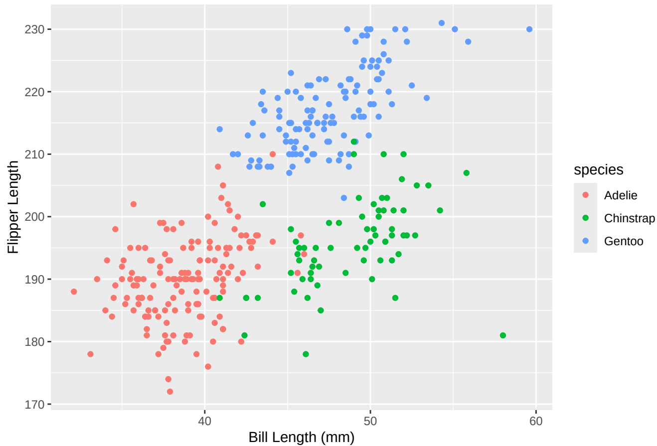
Bill Length vs. Flipper Length
