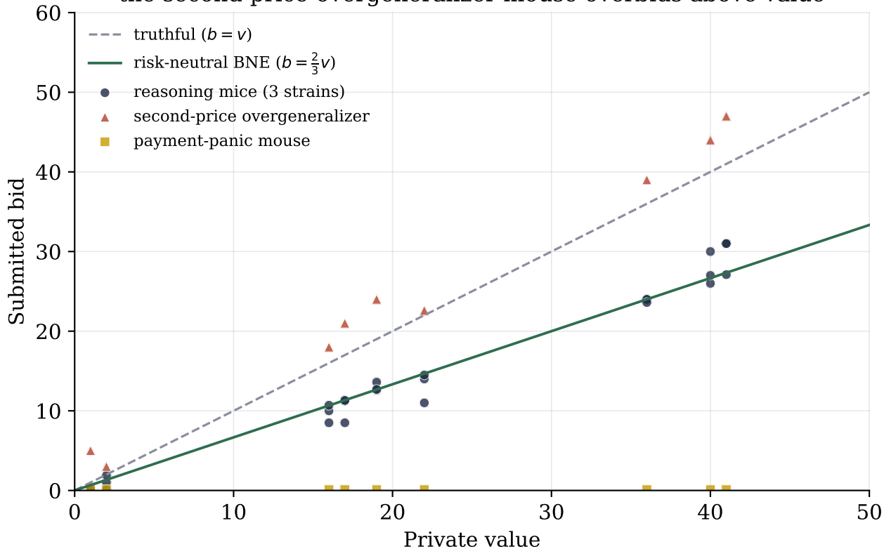
First-price stress test: reasoning mice track the BNE; the second-price-overgeneralizer mouse overbids above value
