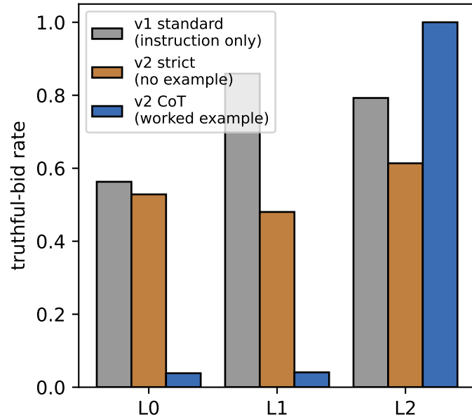
Contingent reasoning
