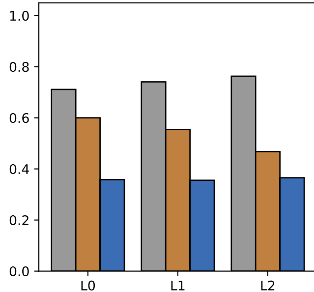
Belief reasoning
