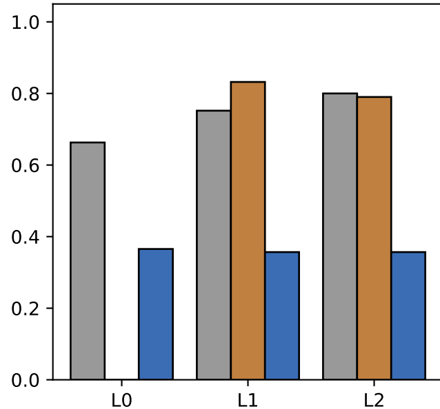
Forward planning
