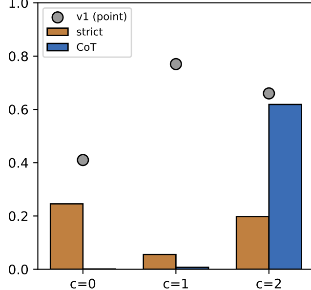
Dominance-invocation rate
