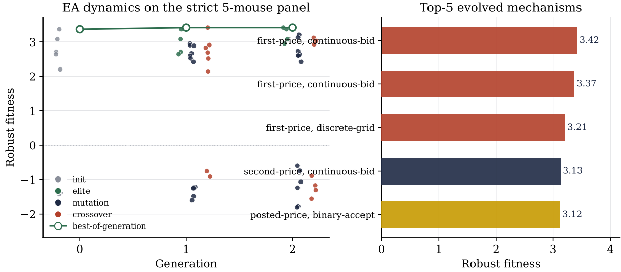
Figure 7: Evolutionary-search dynamics on the 5-strain screening panel. Left: robust fitness of each individual by generation, colored by operator (initialization / mutation / crossover); the green line traces the best-of-generation. Right: the top-five unique evolved mechanisms, colored by payment rule. First-price dominates the top of the population.
