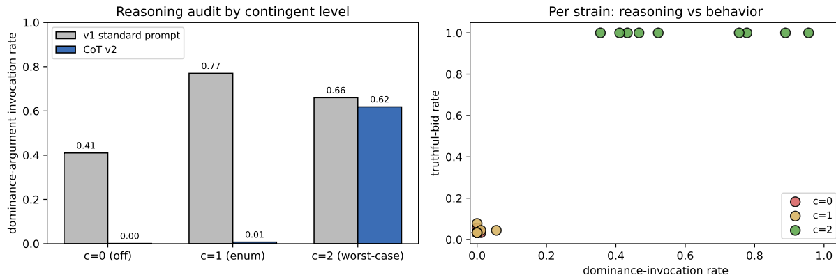
Figure 5: Reading the reasoning chains in the CoT panel. Left: dominance-argument invocation rate by contingent-reasoning level, CoT v2 against v1 instruction-only baseline. The c=0 leak drops from 0.41 to 0.001 once the deficit is induced by demonstration. Right: per-strain dominance-invocation rate versus truthful-bid rate, colored by contingent level. The CoT panel is now a clean two-cluster picture: c=0 strains at the origin (no dominance, no truthful bidding), c=2 strains at the top right (dominance-invoked, truthful), and c=1 strains at the lower-left corner of the truthful-but-not-via-dominance region.
