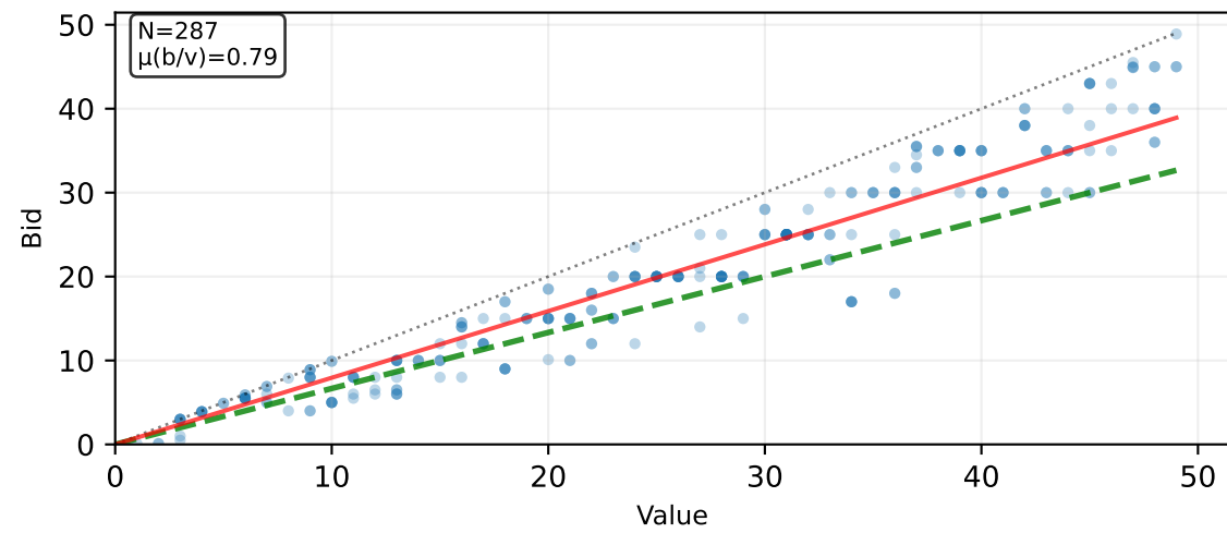
Proxy/Clock - FPSB
