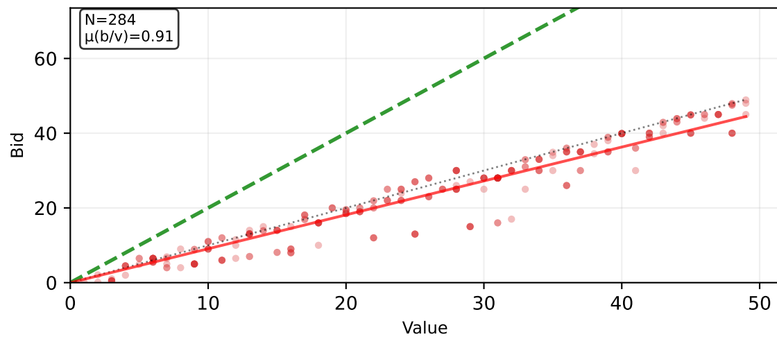
Proxy/Clock - TPSB
