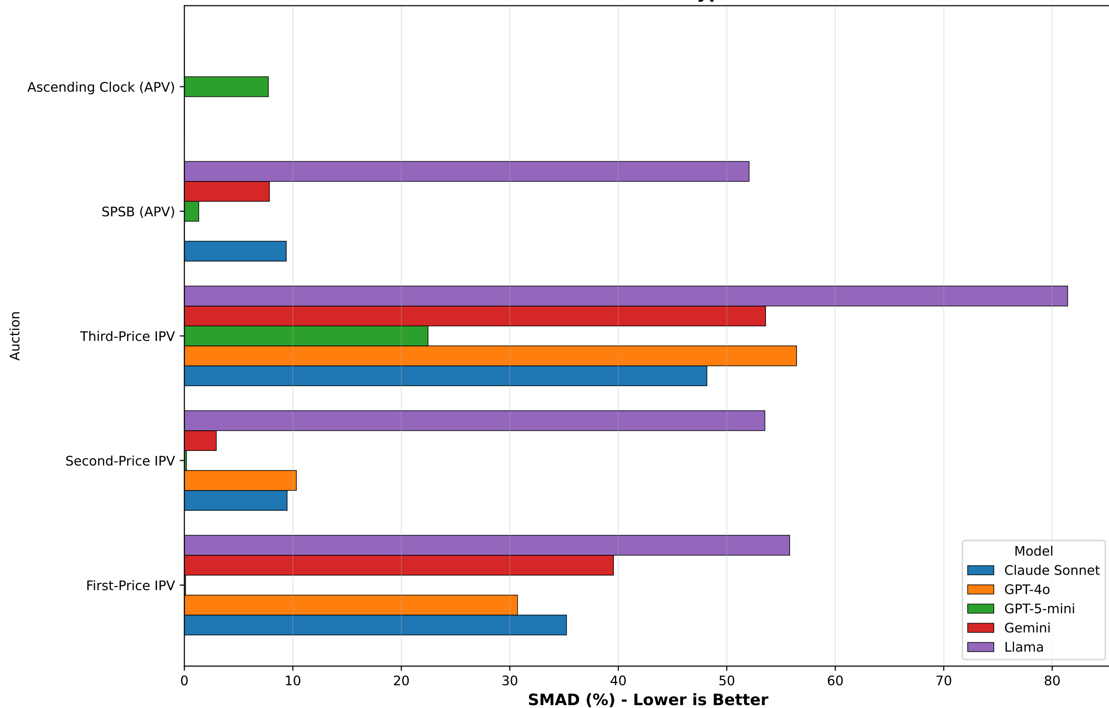
SMAD Across All Auction Types and Models
