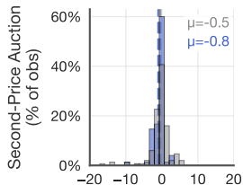
Claude 3.5 Haiku
