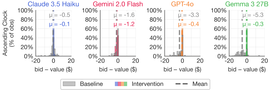
Figure 5: Implementation cell of the design map, per model family. Distribution of bid deviations from value ( \text{bid} - \text{value} ) in the second-price sealed bid (gray, dedicated SPSB cells) and the ascending clock (colored); dashed lines mark means. Every family deviates in the sealed-bid format; the clock corrects every family toward truthful play and removes the left tail of severe underbids. The matching-domain counterpart of this exhibit is in Appendix K (Figure 31).
