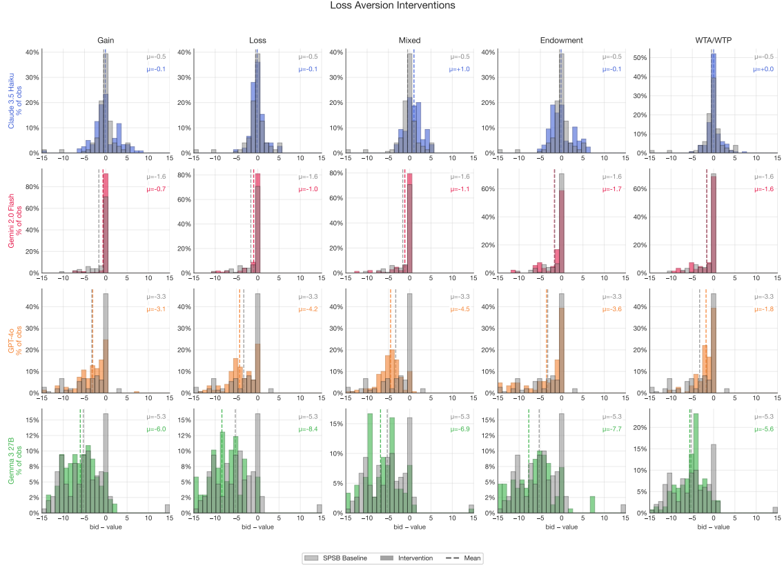
Figure 15: Loss-aversion and framing interventions in SPSB auctions (mean bid deviation from value, $). Baseline SPSB in gray, intervention in color; dashed lines indicate means. None of the framing interventions consistently improve play relative to the SPSB baseline ( \mu = -2.67 ). The loss frame ( \mu = -3.44 ) and endowment ( \mu = -3.40 ) worsen underbidding, while the gain frame ( \mu = -2.51 ) and WTA/WTP ( \mu = -2.17 ) show modest, inconsistent effects.
