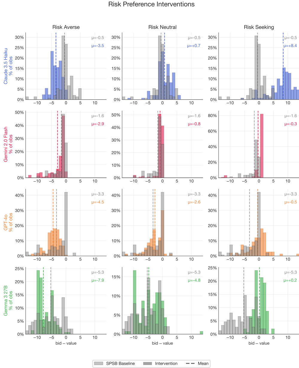
Figure 17: Risk-preference personas in SPSB auctions (mean bid deviation from value, $). Risk aversion increases underbidding ( \mu = -4.71 ), while risk-seeking dramatically shifts Claude 3.5 Haiku to overbidding ( \mu = +8.40 ). Risk neutrality ( \mu = -1.82 ) modestly improves play relative to the SPSB baseline ( \mu = -2.67 ).
