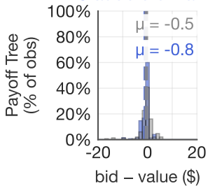
Claude 3.5 Haiku
