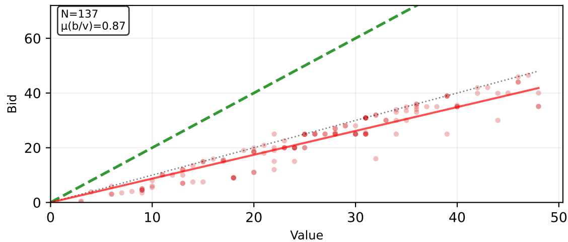
List Cases - TPSB
