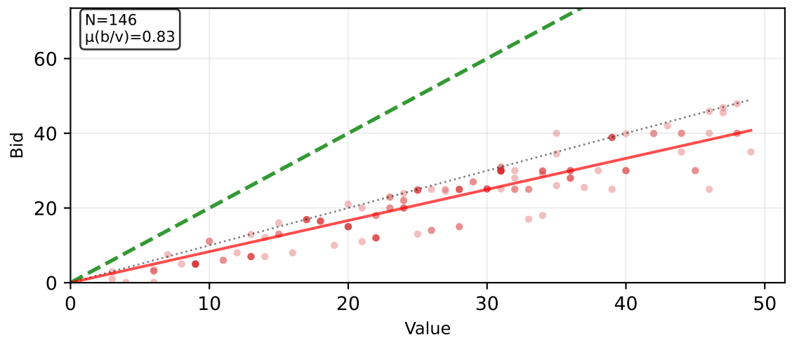
Dominated Bid - TPSB
