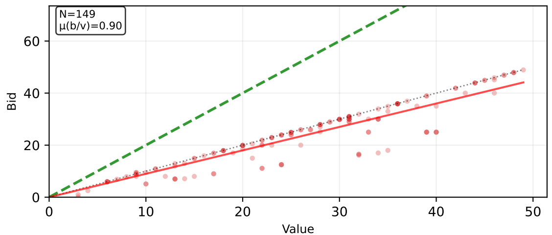
Nash Deviation - TPSB
