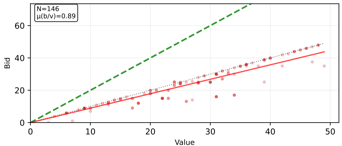
Worst Case - TPSB
