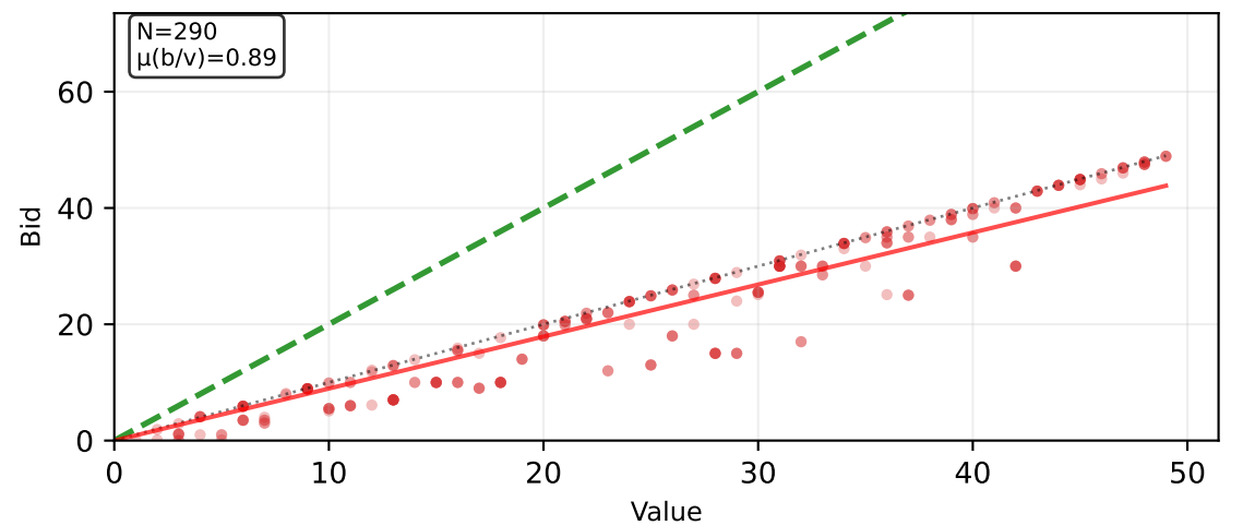
Nash Deviation - TPSB
