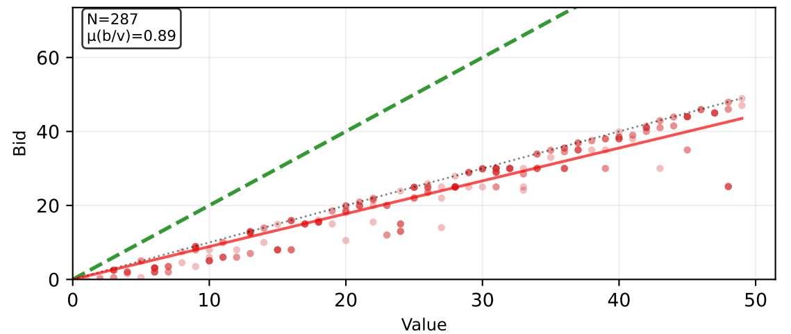
List Cases - TPSB
