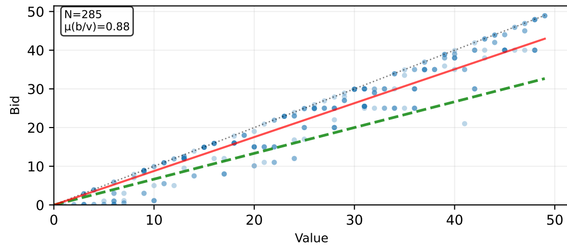
Dominated Bid - FPSB
