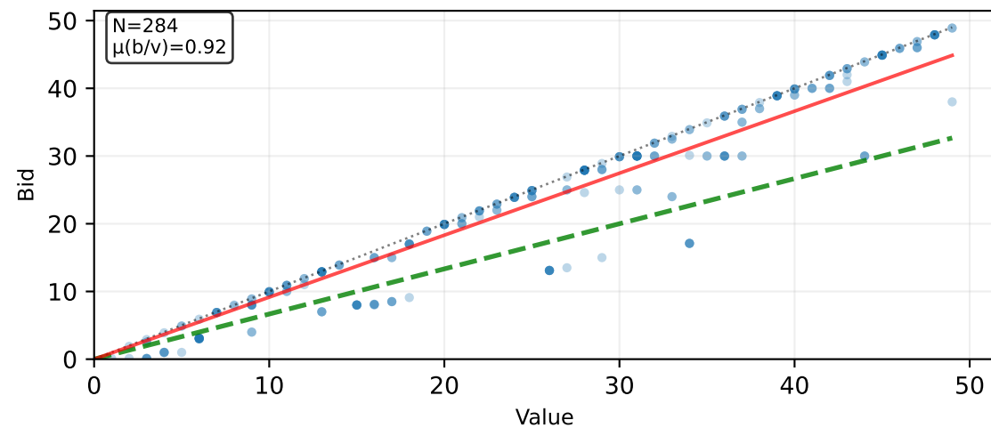
Nash Deviation - FPSB
