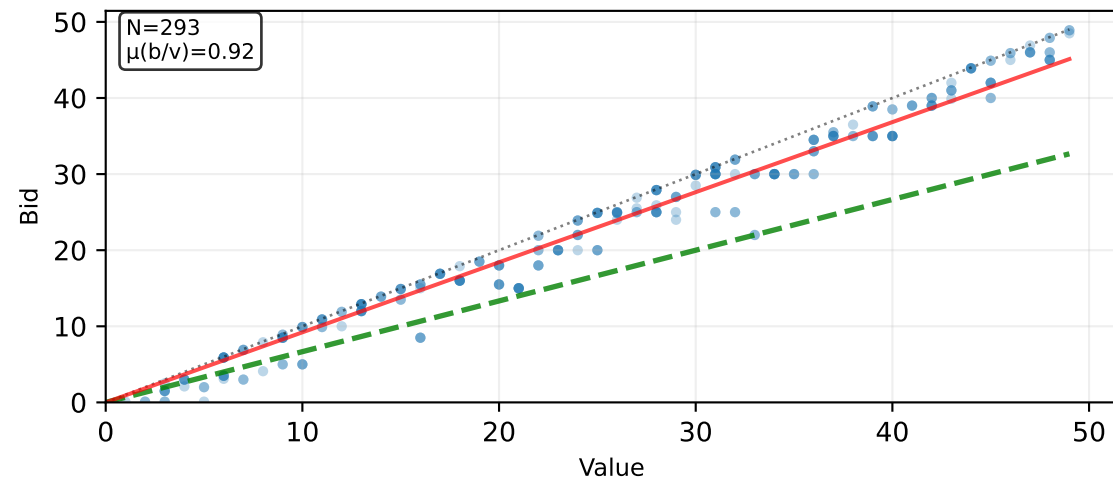
List Cases - FPSB
