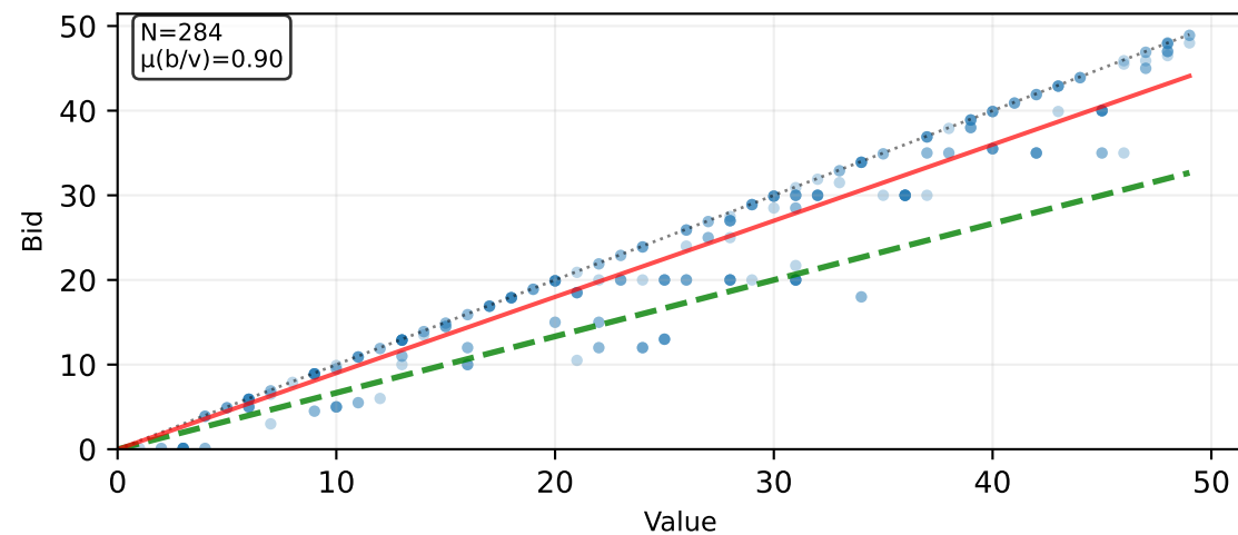
Worst Case - FPSB
