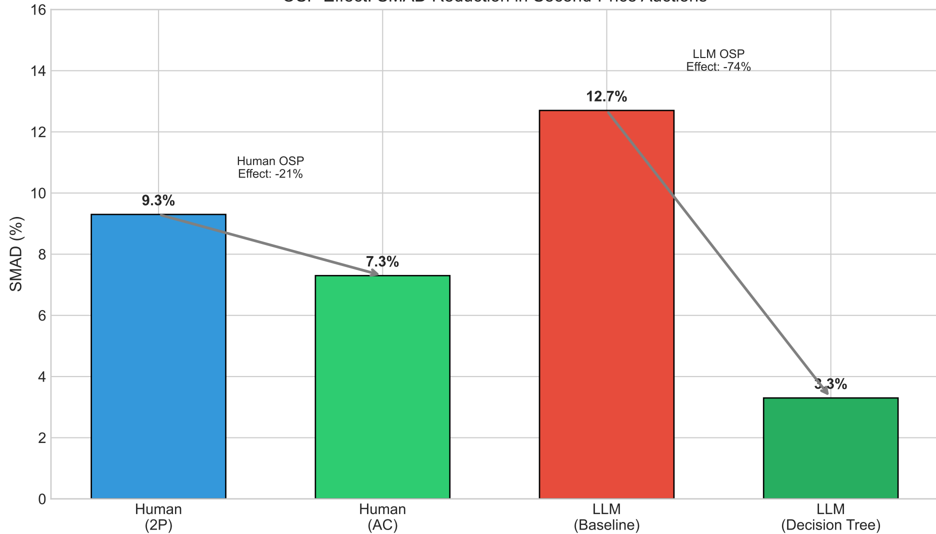
OSP Effect: SMAD Reduction in Second-Price Auctions
