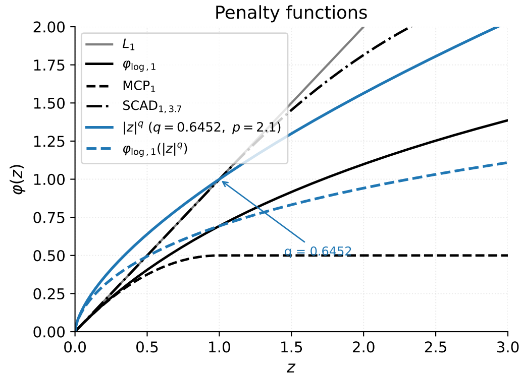
Non-convex penalty functions + power-transformed penalties ( p=2.1 , q=0.6452 )
