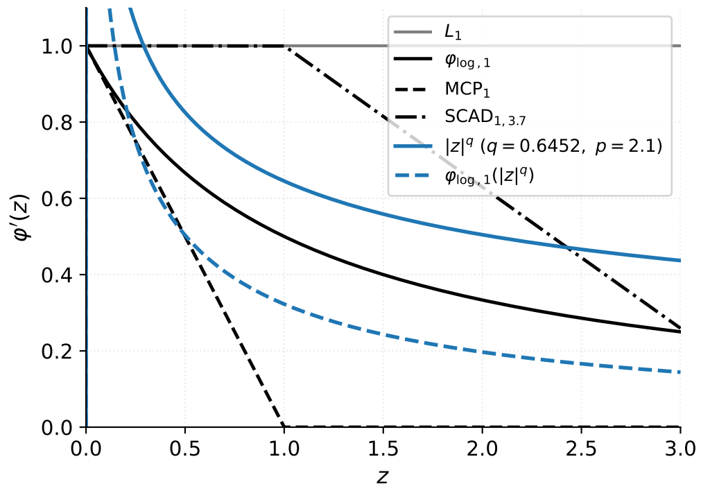
Derivatives
