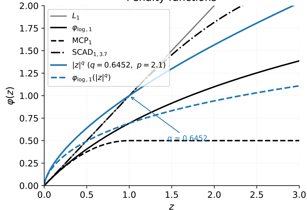
Penalty functions
