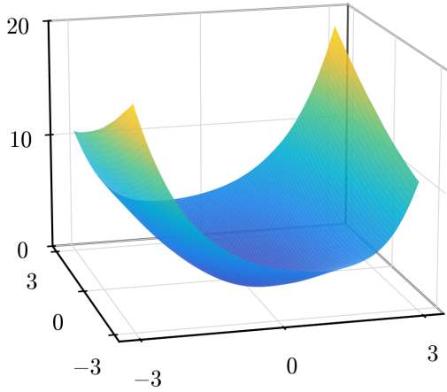
(A) k = 2
