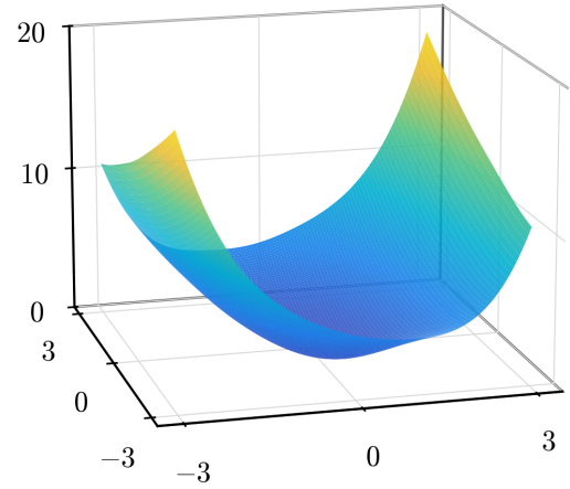
(B) k = 3
