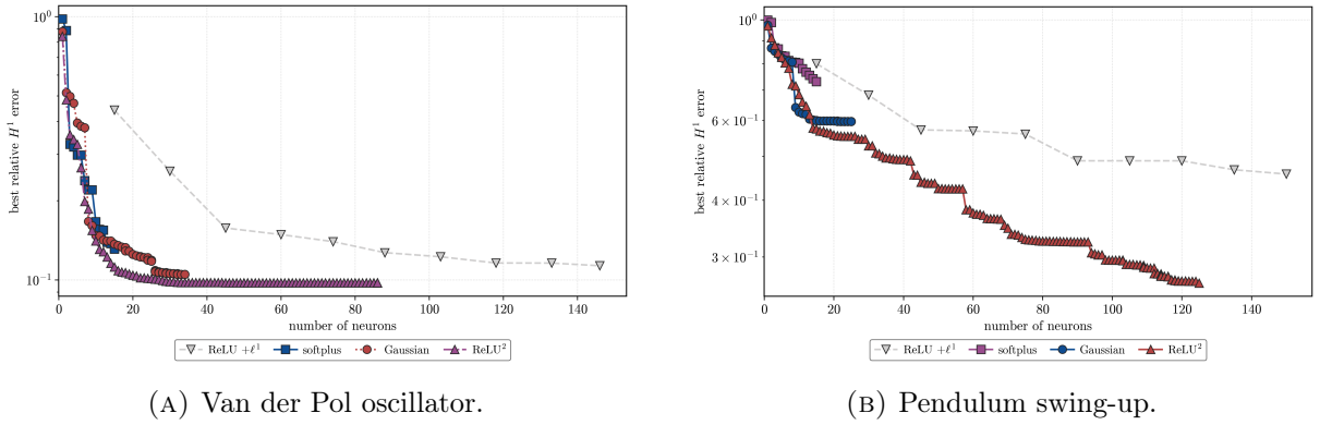
FIGURE 1. Running best relative H^1 validation error as neurons are inserted. The nonhomogeneous activations are fitted by Algorithm 1 at the common operating point (\alpha, \gamma, p) = (10^{-4}, 10, 2.01) ; \text{ReLU}^2 and the \ell^1 baseline are fitted by Algorithm 2, the latter at k = 1 , where the induced exponent is q = 1 . All curves use one atom per outer iteration and seed 42.
