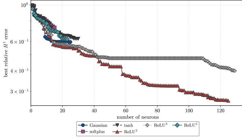
FIGURE 14. Best relative H^1 validation error against neuron count. The non-homogeneous activations use (64); the homogeneous activations use J_{\psi_k}^M with \alpha = 10^{-6} for k \in \{2, 3\} and \alpha = 10^{-4} for k = 5 .
