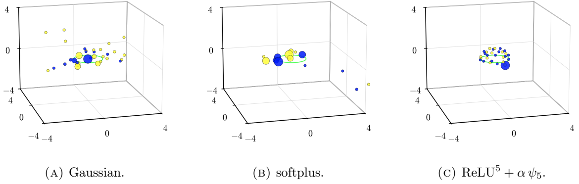
FIGURE 9. Inner parameters (a_1, a_2, b) , with the unit circle in the plane b = 0 shown in light green. The two nonhomogeneous fits use the common operating point \alpha = 10^{-4} , \gamma = 10 , p = 2.01 ; dot color gives the sign and dot size the magnitude of the outer weight.
