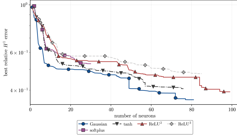
FIGURE 14. Best relative H^1 validation error against neuron count. The non-homogeneous activations use (56); the homogeneous activations use J_{\psi_k}^M with \alpha = 10^{-5} for k = 2 and \alpha = 10^{-6} for k = 3 .
