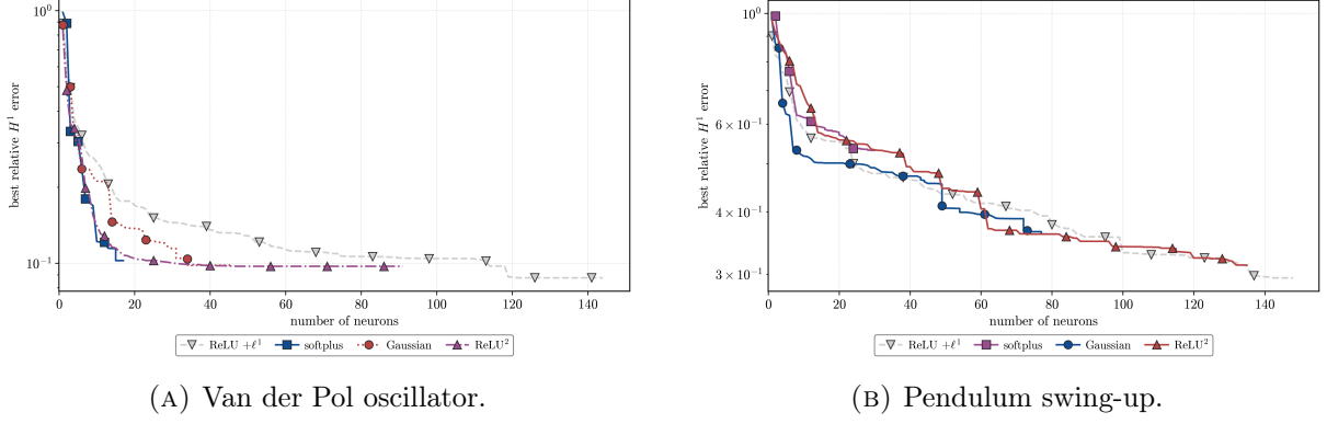
FIGURE 1. Running best relative H^1 validation error as neurons are inserted. The nonhomogeneous activations are fitted by Algorithm 1 with (\alpha, \gamma, p) = (10^{-4}, 10, 2.01) ; \text{ReLU}^2 and the traditional \ell^1 network are fitted by Algorithm 2, the latter at k = 1 , where the induced exponent is q = 1 . All curves use one atom per outer iteration and seed 42.
