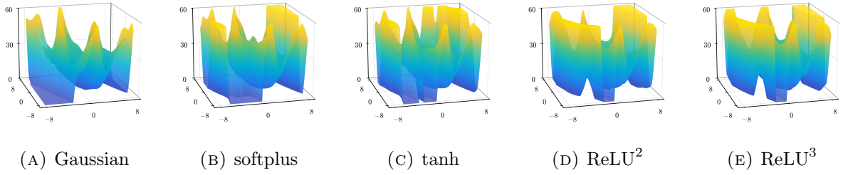
FIGURE 11. Learned value surfaces \hat{V}(x) over the (\theta, \dot{\theta}) window [-8, 8]^2 . Predictions below 0 or above 60 are clipped to the respective boundary for visualization; errors and feedback use the unclipped fitted function. The \text{ReLU}^k models are trained with the fractional-exponent penalty \psi_k , and the nonhomogeneous models with (56) using the parameter values reported in Figure 1b.
