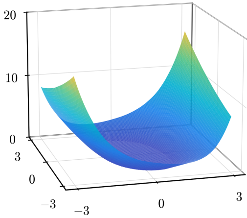
(A) k = 2 ( N = 53 , \text{Err}_{H^1} = 0.235 ).
