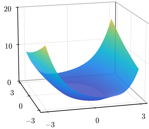
(B) k = 3 ( N = 26 , \text{Err}_{H^1} = 0.235 ).
