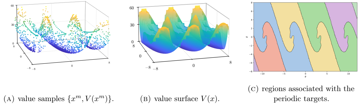
FIGURE 10. Optimal value function V(x) over the (\theta, \dot{\theta}) plane, 2\pi -periodic in \theta . (a) The raw (x, V) samples produced by the PMP generator. (b) The reconstructed value surface. (c) Regions where V_0 or another periodic fixed-target value is minimal; their boundaries form S , across which \nabla V may be discontinuous.
