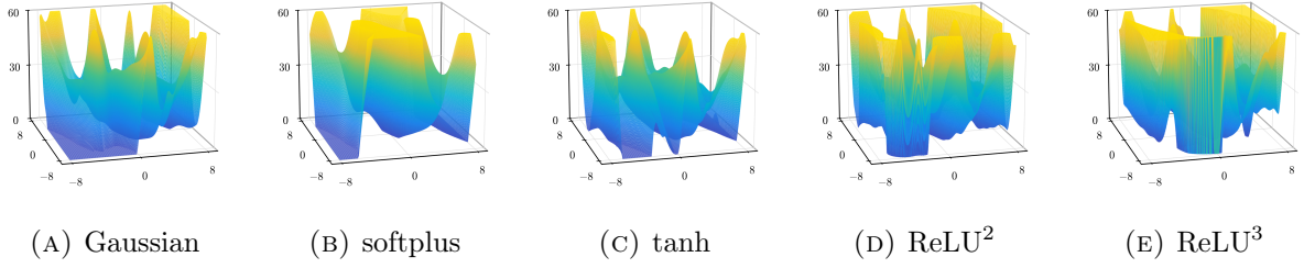
FIGURE 11. Learned value surfaces \hat{V}(x) over the (\theta, \dot{\theta}) window [-8, 8]^2 , displayed on the common range \hat{V} \in [0, 60] . The \text{ReLU}^k models are trained with the fractional-exponent penalty \psi_k , and the nonhomogeneous models with (56) using the parameter values reported in Figure 1b.
