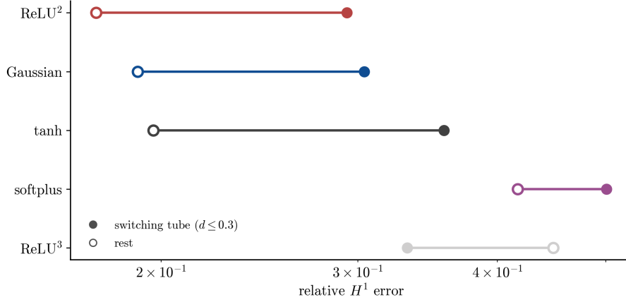
FIGURE 14. Relative H^1 error on S_{0.3} (filled markers) and D \setminus S_{0.3} (open markers), with rows ordered by the latter error.
