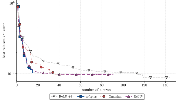
(A) Van der Pol accuracy against width.
