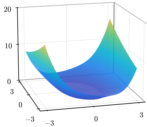
(B) k = 3 ( N = 28 , \text{Err}_{H^1} = 0.099 ).
