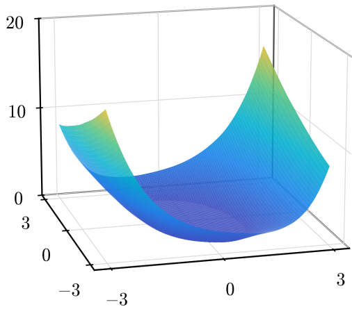
(A) k = 2 ( N = 45 , \text{Err}_{H^1} = 0.099 ).
