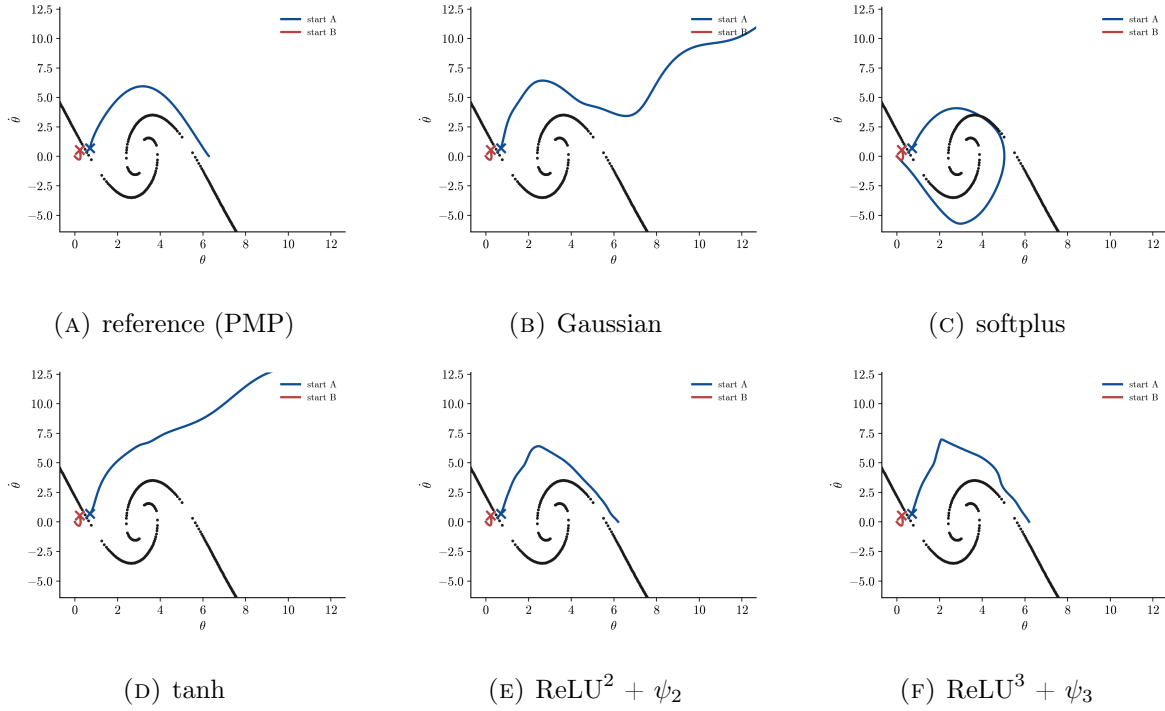
FIGURE 15. Closed-loop paths in the (\theta, \dot{\theta}) plane from the two starts A (blue) and B (red) on either side of the switching curve (black), one panel per feedback law; all panels share the same axes. The reference law swings over the top from A and brakes to \theta = 0 from B . Softplus, \text{ReLU}^2 , and \text{ReLU}^3 reach an upright neighbourhood from both starts; the Gaussian and tanh reach one only from B .
