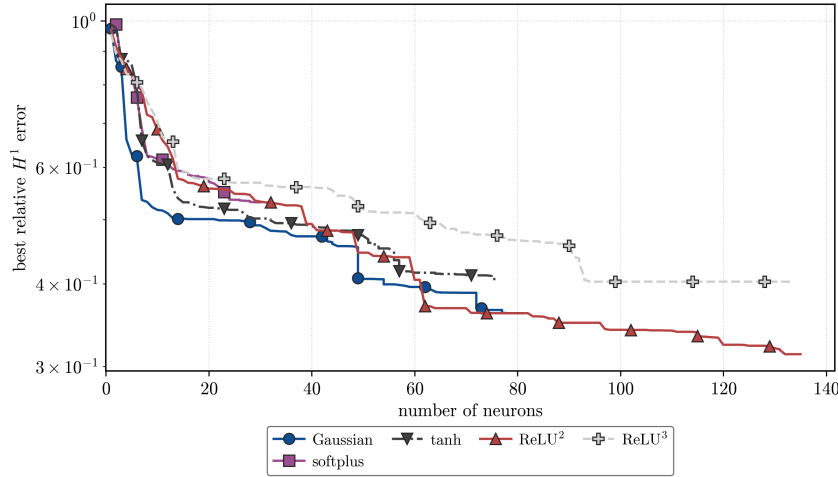
FIGURE 13. Best relative H^1 validation error against neuron count. The non-homogeneous activations use (56); the homogeneous activations use J_{\psi_k}^M with \alpha = 10^{-6} for both k = 2 and k = 3 .
