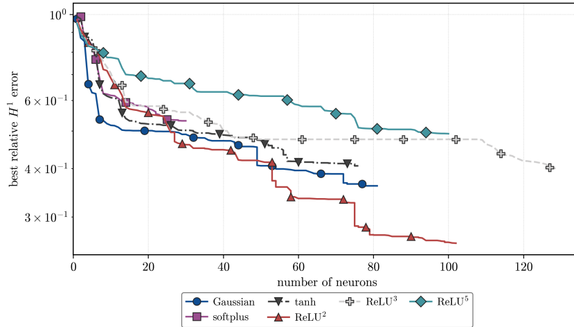
FIGURE 14. Best relative H^1 validation error against neuron count. The non-homogeneous activations use (64); the homogeneous activations use J_{\psi_k}^M with \alpha = 10^{-5} for k = 2 and \alpha = 10^{-6} for k \in \{3, 5\} .
