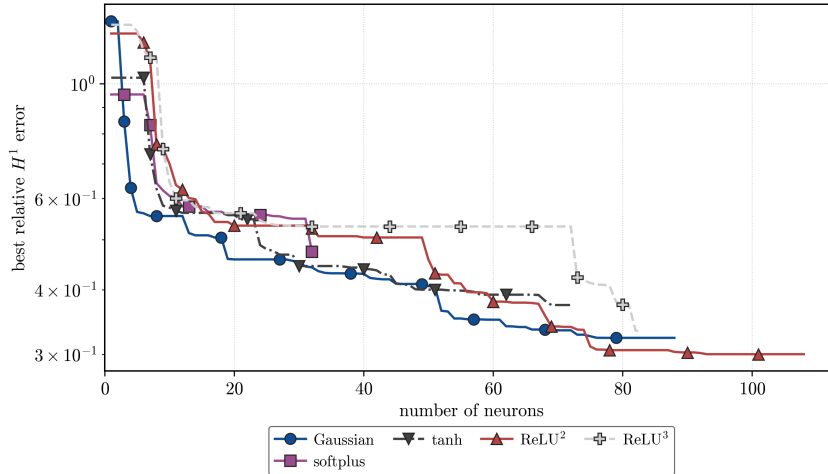
FIGURE 13. Best relative H^1 validation error against neuron count. The non-homogeneous activations use (56); the homogeneous activations use J_{\psi_k}^M with \alpha = 10^{-5} for both k = 2 and k = 3 .
