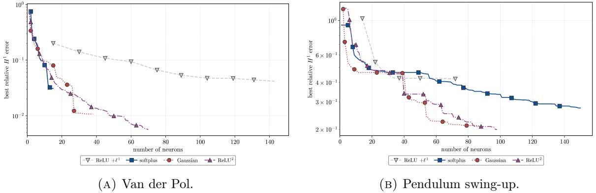
FIGURE 1. Best observed relative H^1 validation error at each support budget for (a) Van der Pol and (b) Pendulum swing-up. See Sections 6.1 and 6.2 for the experimental settings.
