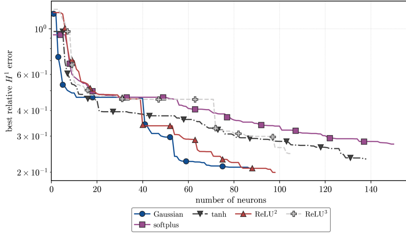
FIGURE 10. Best relative H^1 validation error against neuron count. The nonhomogeneous activations use (48); the homogeneous activations use J_{\psi_k} . All curves use the selected runs and parameters in Table 4.
