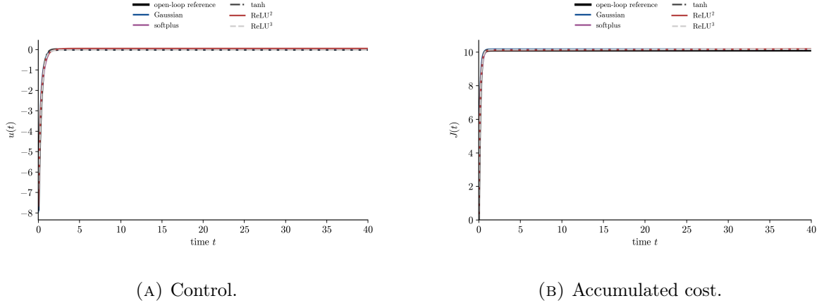
FIGURE 13. Pendulum controls and realized costs from B = (0.26, 0.46) .
