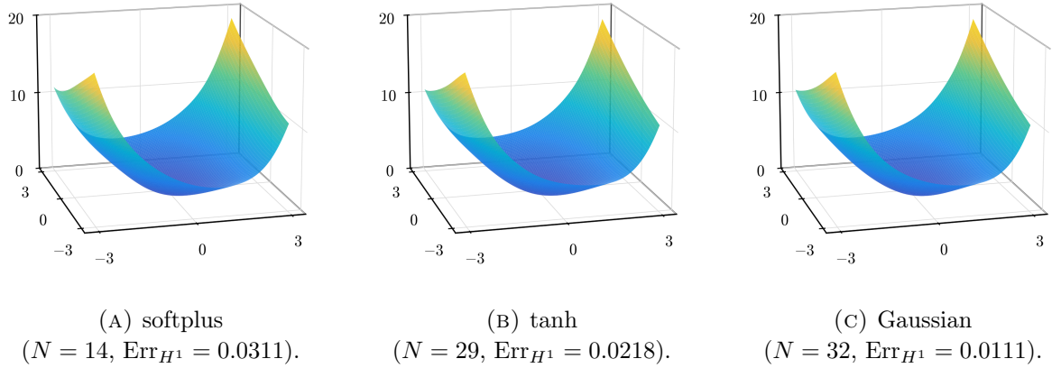
FIGURE 4. Learned value functions under the H^1 loss using the parameter values in Table 1. Predictions are clipped to [0, 20] for visualization.
