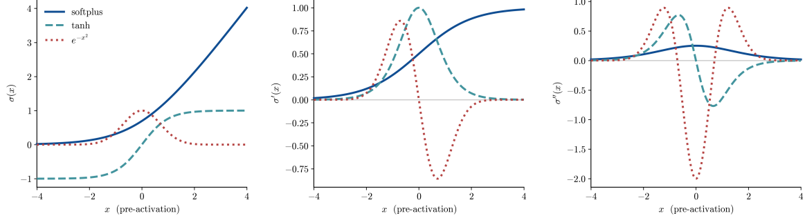
FIGURE 3. The three smooth profiles used by Algorithm 1 — softplus, tanh, and the Gaussian e^{-x^2} — shown as \rho , \rho' , and \rho'' . Under the gradient-augmented loss, the first derivative is the basis that reconstructs \nabla V .
