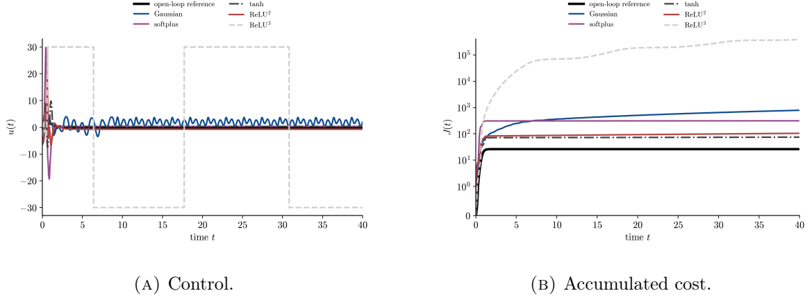
FIGURE 12. Pendulum controls and realized costs from A = (0.74, 0.61) .
