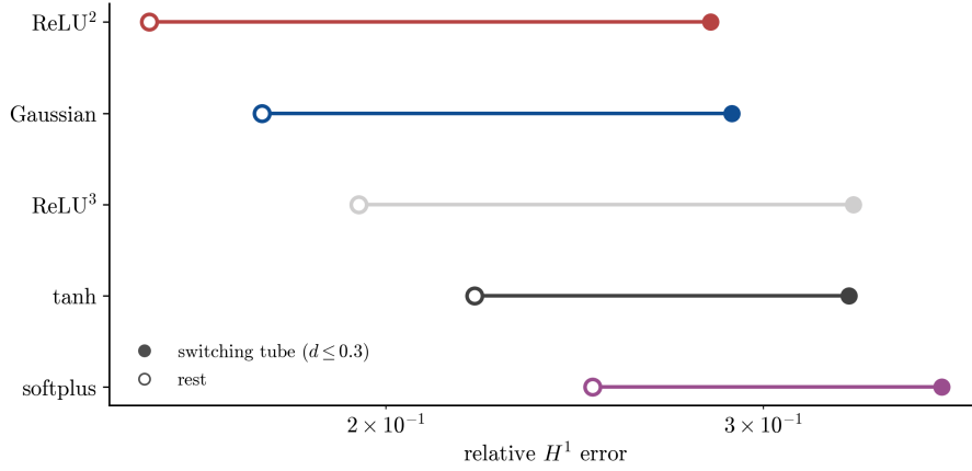
FIGURE 14. Relative H^1 error near the gradient discontinuity (within distance 0.3 of S , filled markers) and on the remaining evaluation points (open markers), with rows ordered by the latter error.
