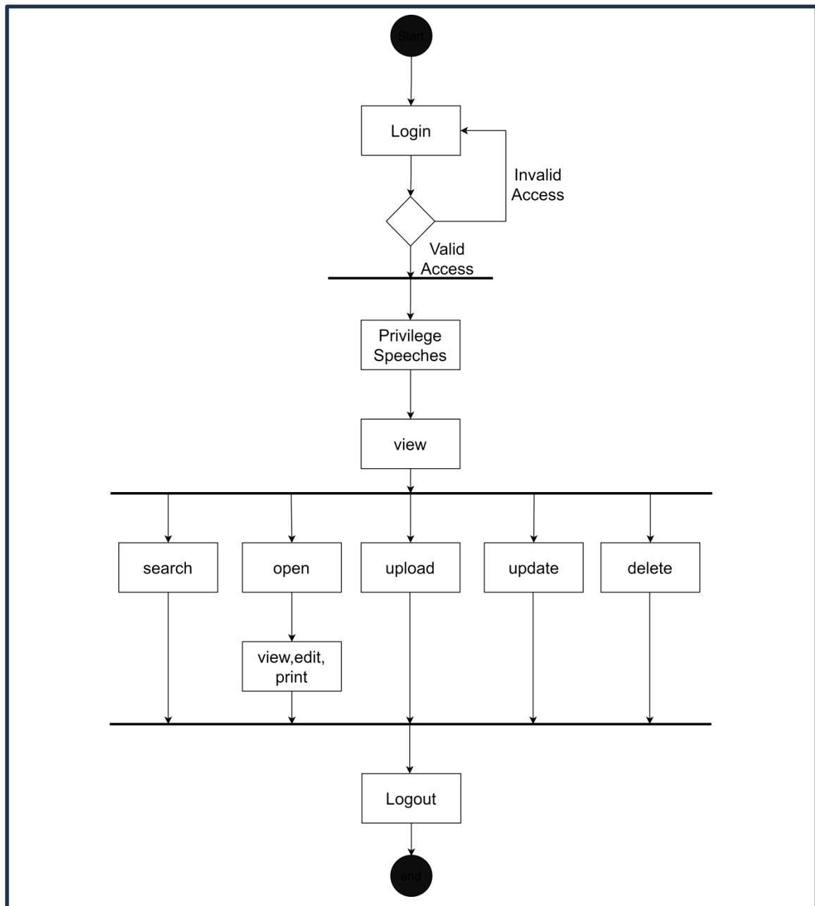
Figure 25. Activity Diagram of the System
