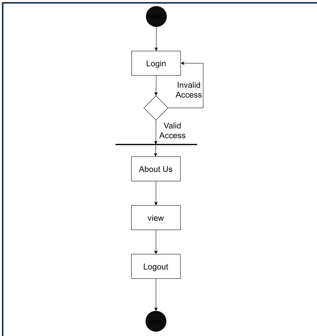
Figure 30. Activity Diagram of the System
