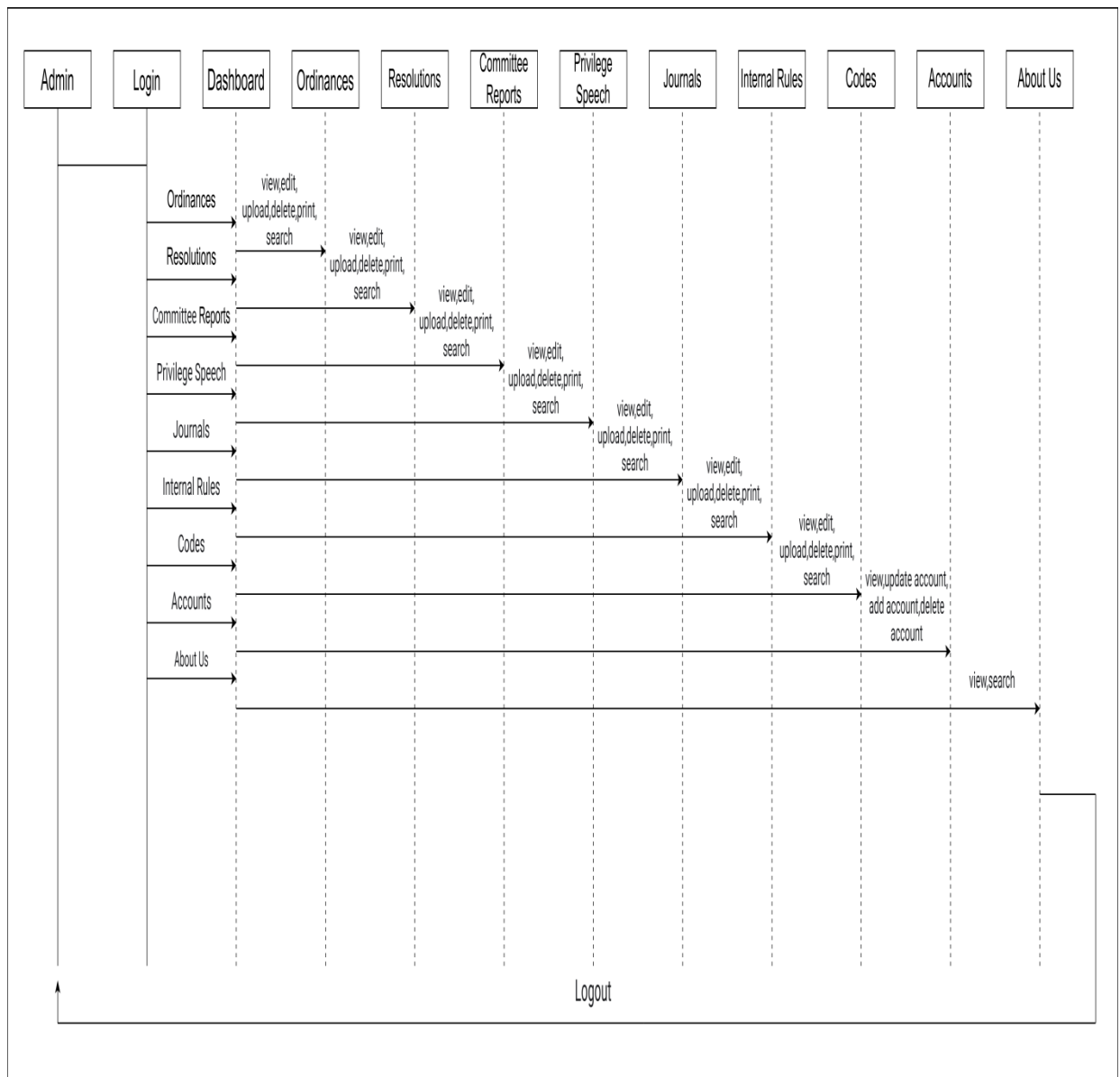
Figure 21. Sequence Diagram - Admin
