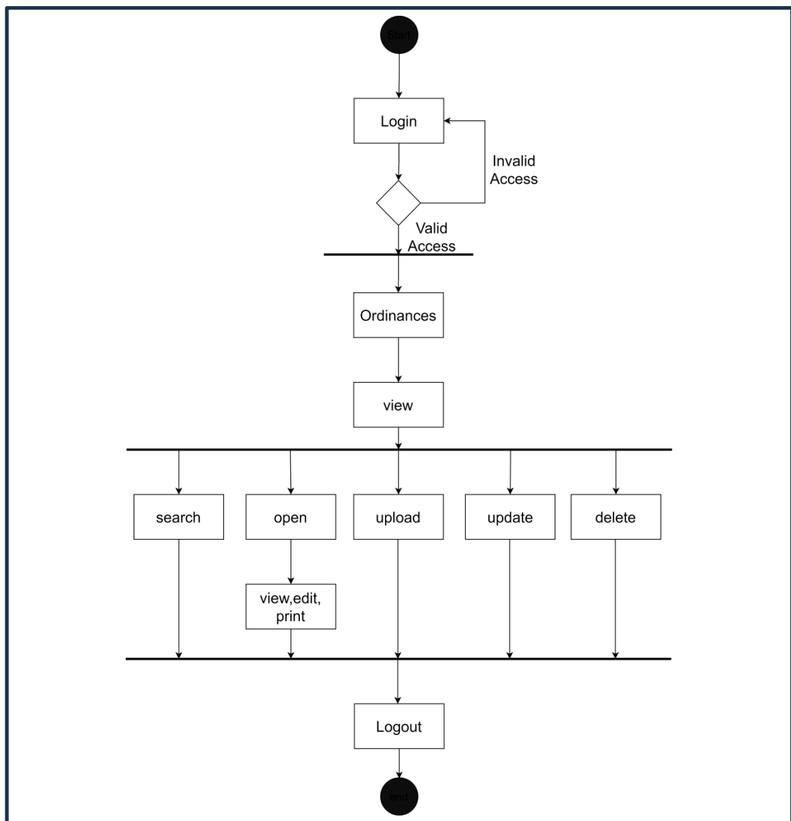
Figure 23. Activity Diagram of the System
