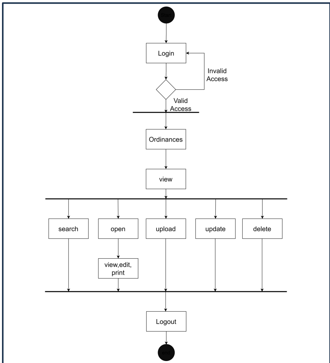
Figure 24. Activity Diagram of the System
