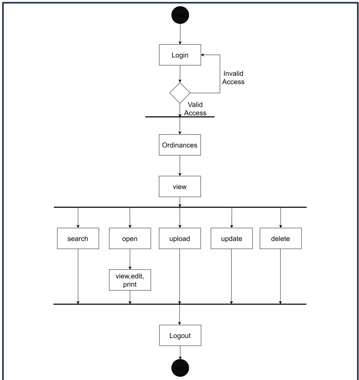
Figure 28. Activity Diagram of the System
