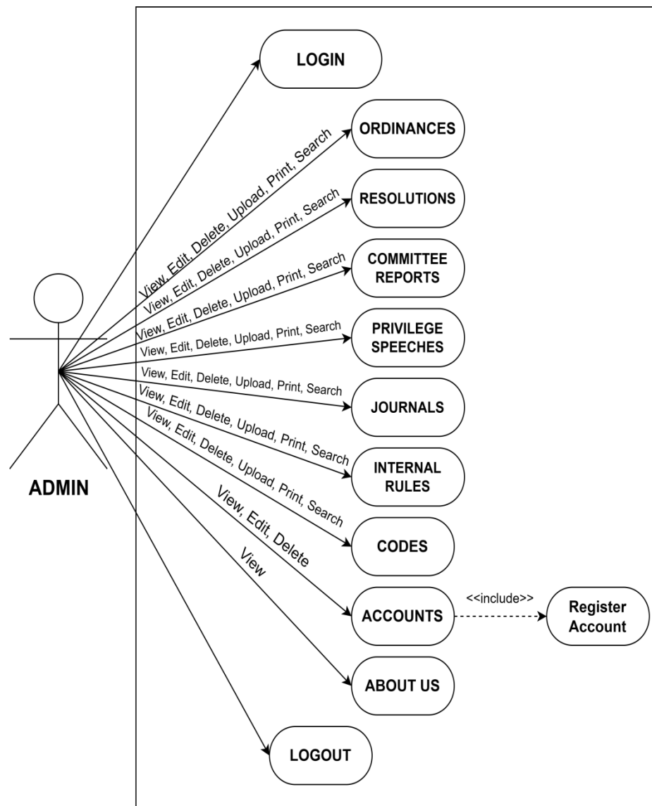
Figure 19. Use Case Diagram of the System - Admin
