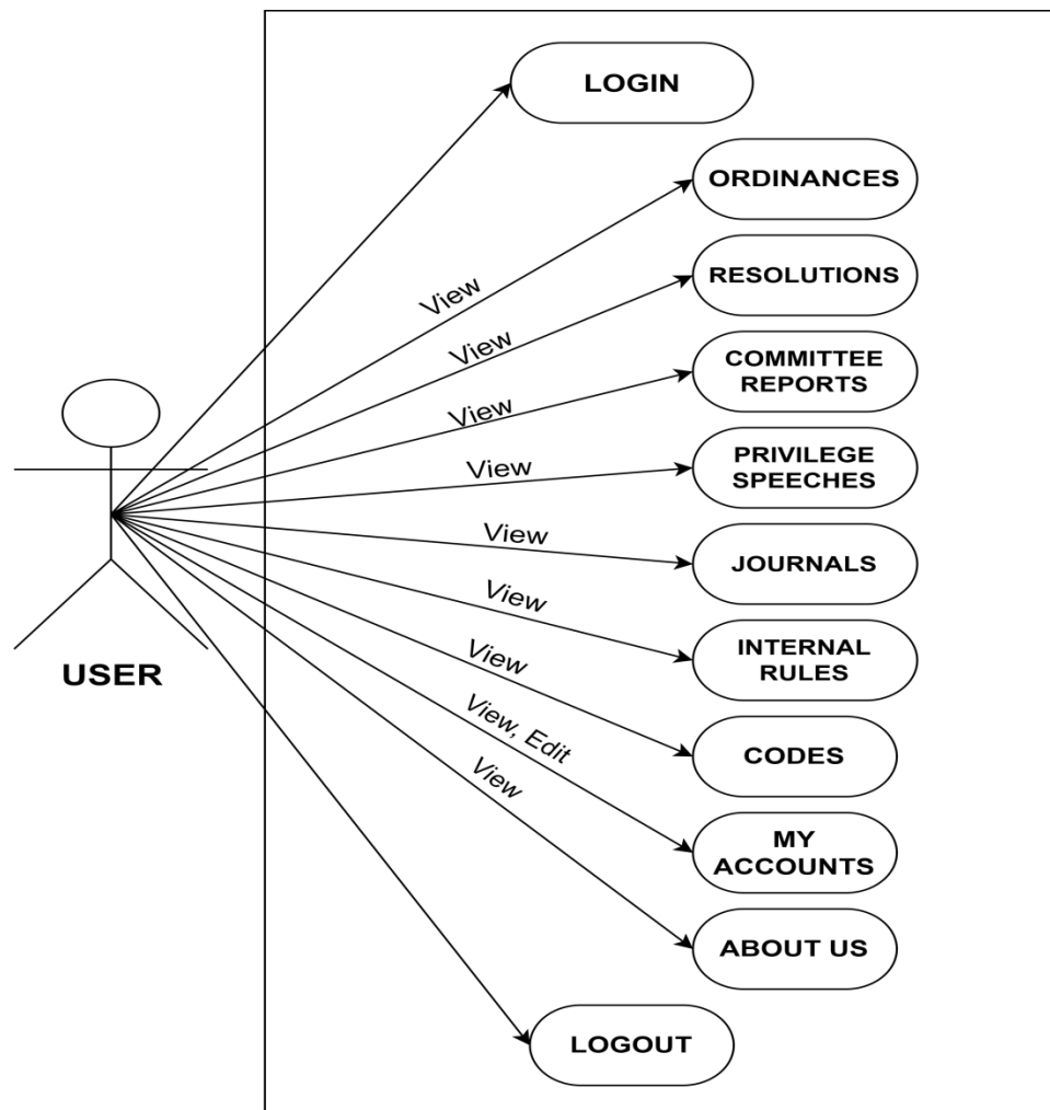
Figure 20. Use Case Diagram of the System - User
