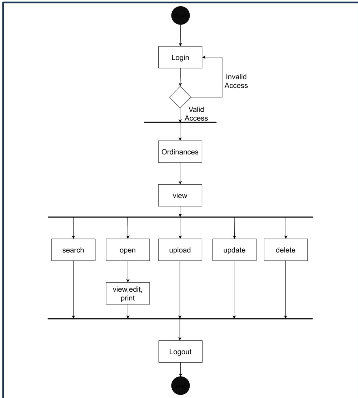
Figure 26. Activity Diagram of the System
