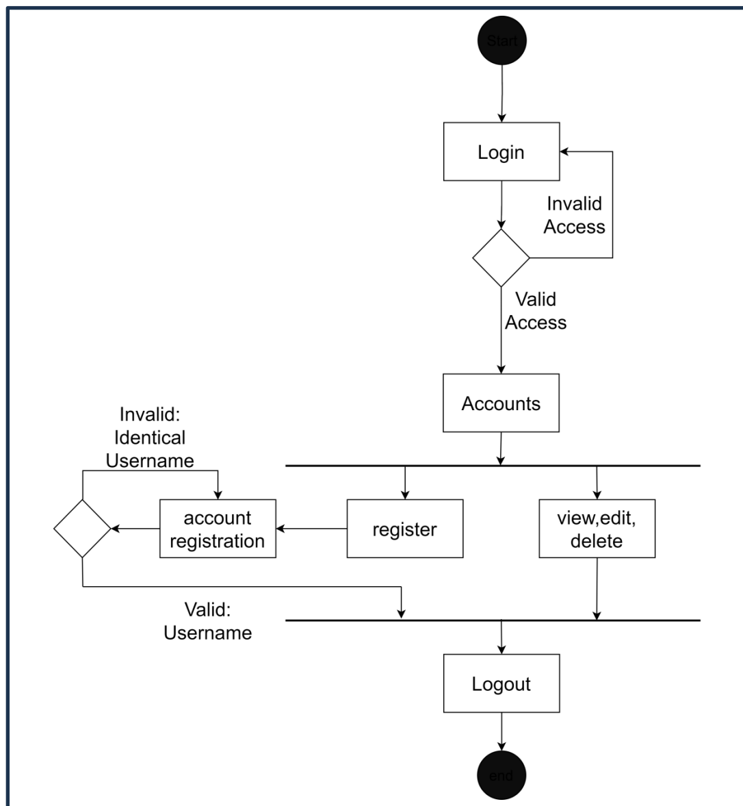
Figure 29. Activity Diagram of the System
