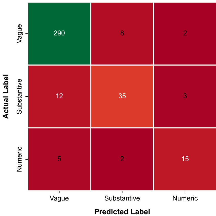
Figure 1: Confusion Matrix — Naive Bayes Classifier
