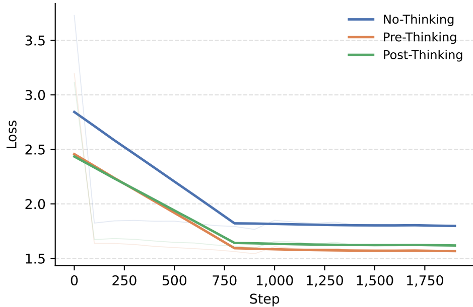
Validation Loss
