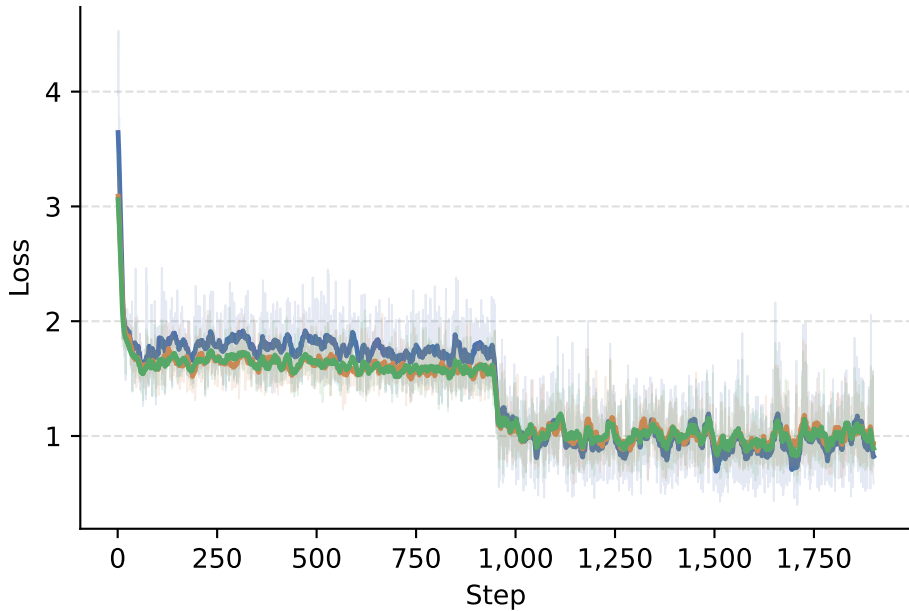
Train Loss
