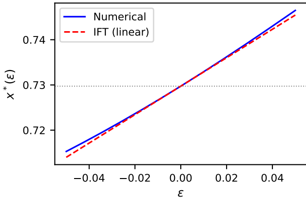
Non-trivial FP x_1^*
