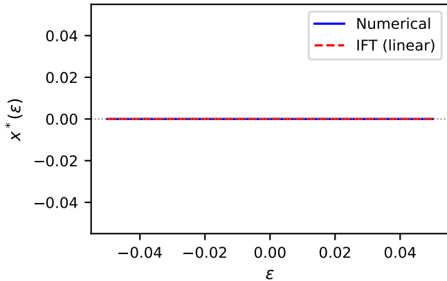
Trivial FP x_0^*
