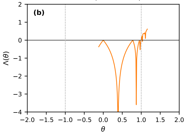
a = 4.0 (fully chaotic)
