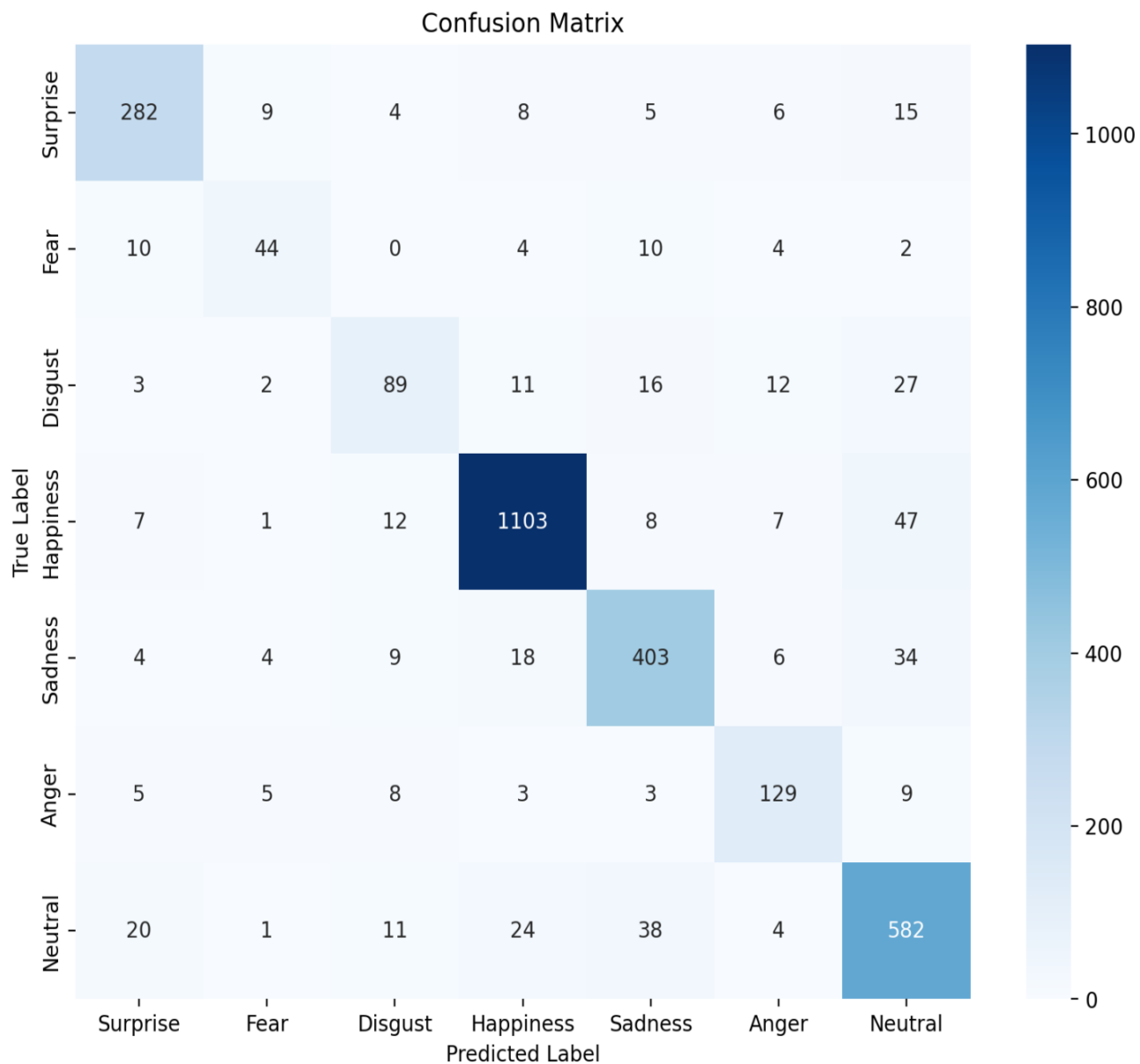
4.4 confusion matrix
