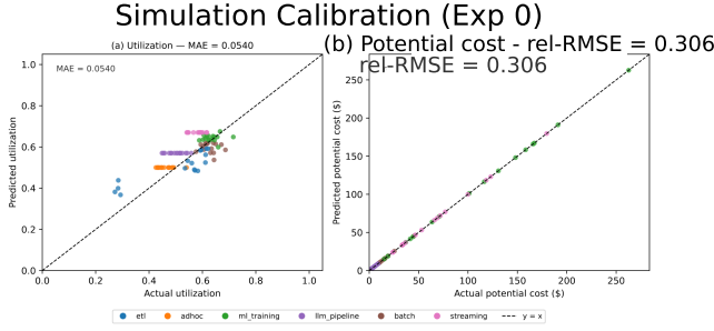
Figure 2: Simulation calibration for Exp 0. Predicted utilization tracks observed utilization closely, with utilization MAE of 0.054; the committed benchmark artifact also reports cost calibration on the same sample.
