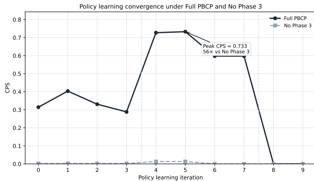
Figure 6: Policy-learning convergence in Exp 6. Full PBCP reaches peak CPS of 0.733, compared with 0.013 for the No Phase 3 baseline, demonstrating a 56× improvement at peak.
