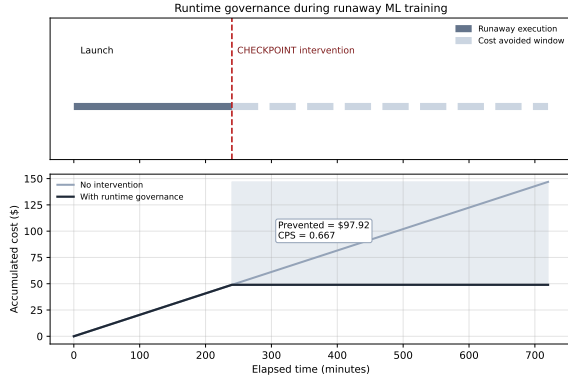
Figure 4: Runtime governance intervention during a runaway ML training workload. The intervention checkpoints prolonged execution at the anomaly boundary, preventing $97.92 of additional cost accumulation.
